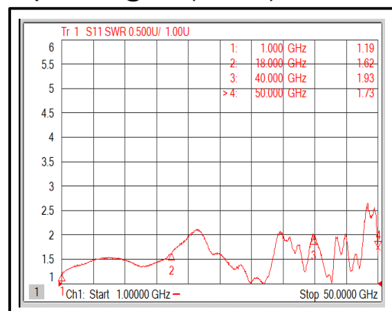
Input VSWR@-40°C (1-50GHz)
