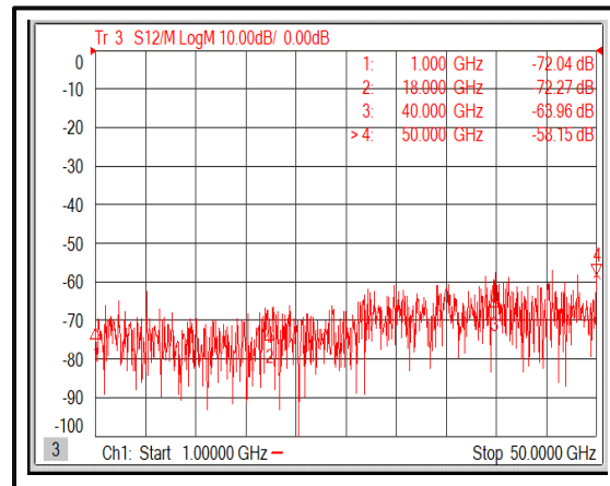
Isolation@-40°C (1-50GHz)
