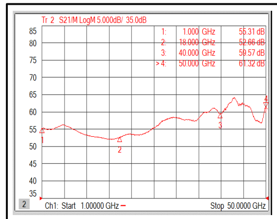
Gain@-40°C (1-50GHz)
