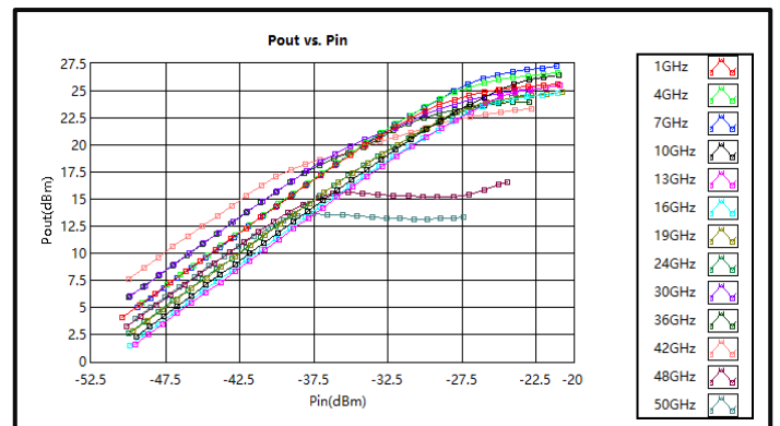
Pout vs. Pin (1-50GHz)
