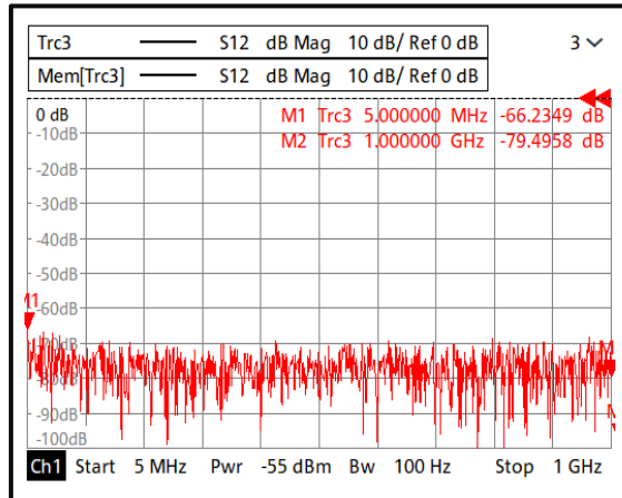
Isolation@+25°C (0.005-1GHz)
