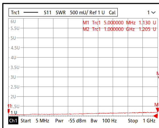
Input VSWR@-40°C (0.005-1GHz)
