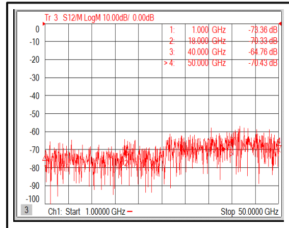
Isolation@+25°C (1-50GHz)
