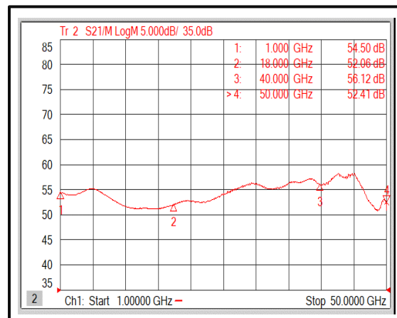
Gain@+25°C (1-50GHz)
