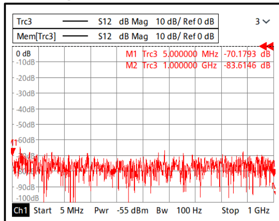
Isolation@-40°C (0.005-1GHz)
