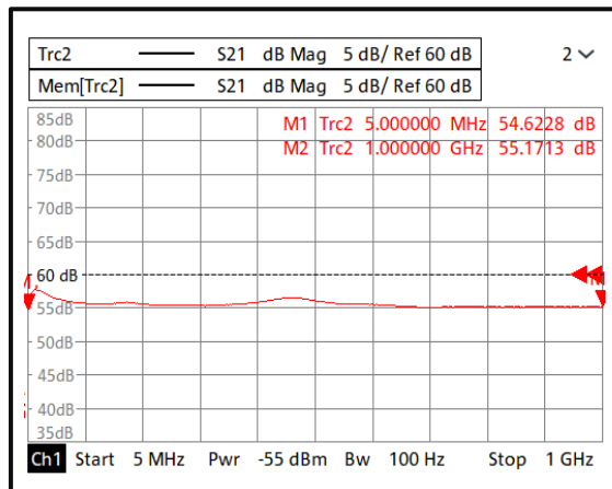
Gain@-40°C (0.005-1GHz)
