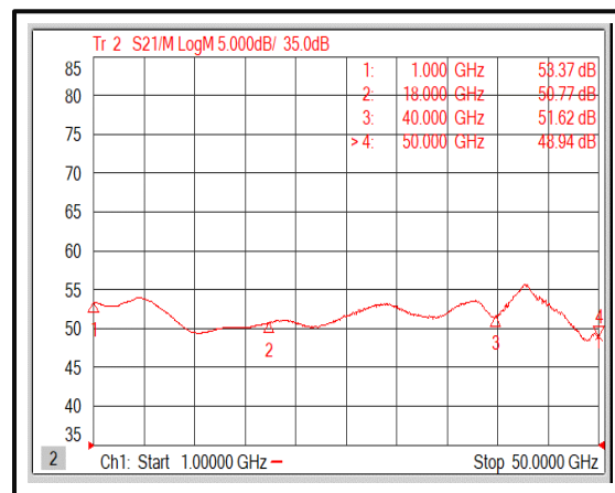
Gain@+85°C (1-50GHz)
