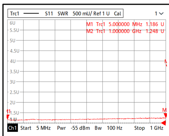
Input VSWR@+25°C (0.005-1GHz)
