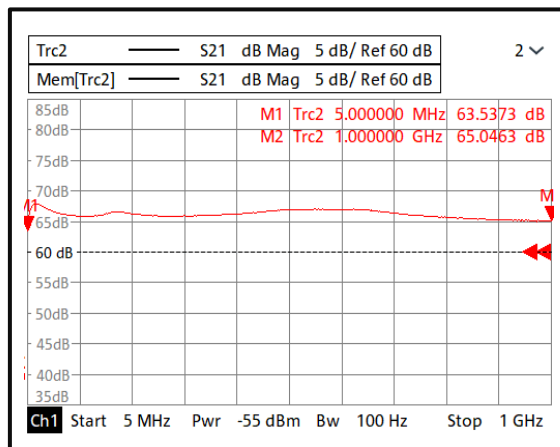
Gain@+25°C (0.005-1GHz)
