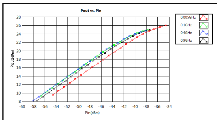
Pout vs. Pin (0.005-0.9GHz)
