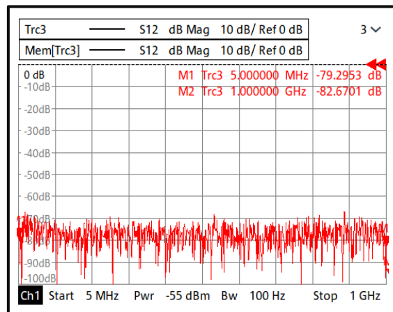
Isolation@+85°C (0.005-1GHz)
