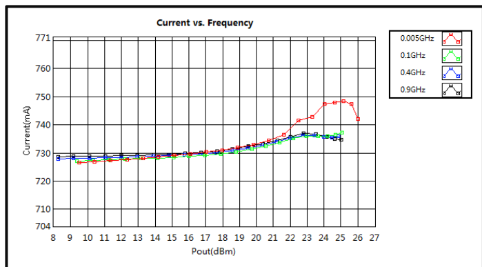
Current vs. Pout (0.005-0.9GHz)
