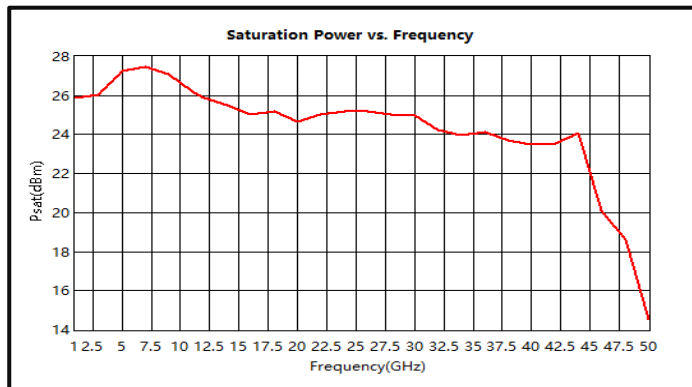
Saturation Power vs. Frequency (1-50GHz)
