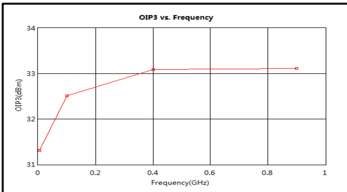
Output Third Order Intercept (OIP3) (0.005-0.9GHz)
