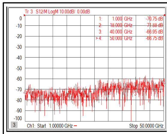
Isolation@+85°C (1-50GHz)
