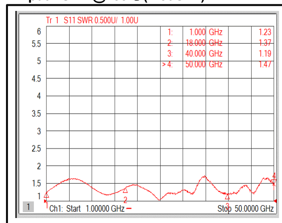
Input VSWR@+85°C (1-50GHz)
