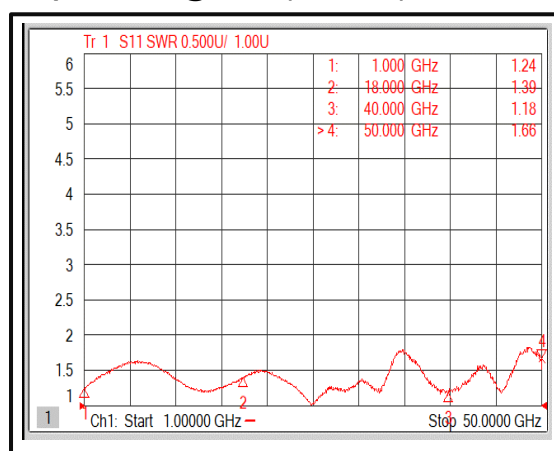
Input VSWR@+25°C (1-50GHz)
