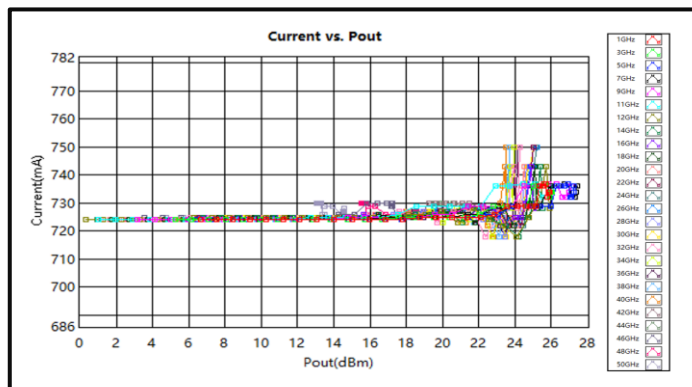
Current vs. Pout (1-50GHz)
