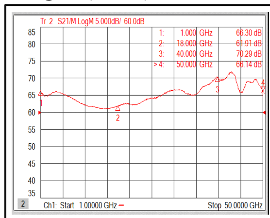
Gain@-40°C (1-50GHz)
