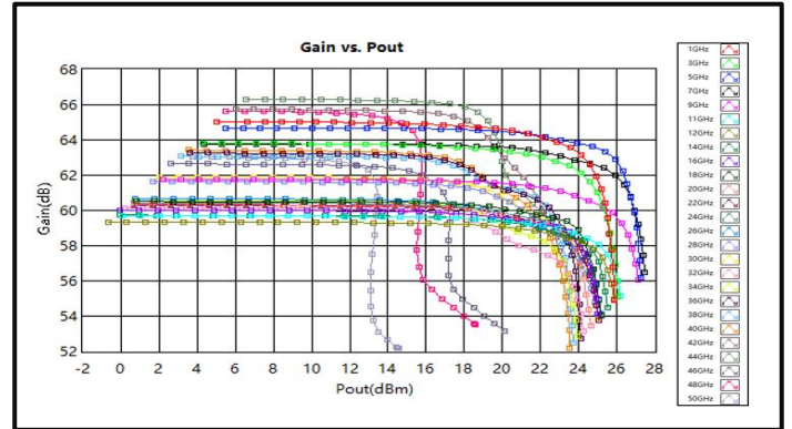
Gain vs. Output Power (1-50GHz)
