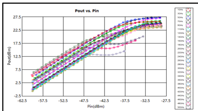
Pout vs. Pin (1-50GHz)
