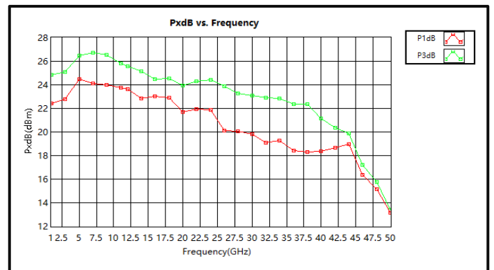
PndB vs. Frequency (1-50GHz)
