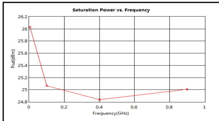
Saturation Power vs. Frequency (0.005-0.9GHz)
