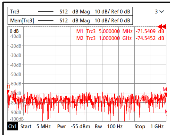
Isolation@+25°C (0.005-1GHz)
