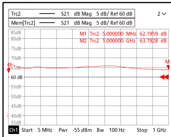
Gain@+85°C (0.005-1GHz)
