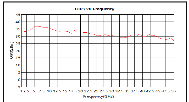
Output Third Order Intercept (OIP3) (1-50GHz)
