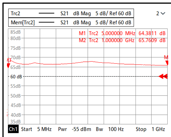
Gain@-40°C (0.005-1GHz)
