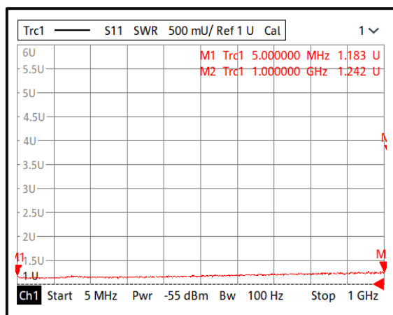
Input VSWR@-40°C (0.005-1GHz)
