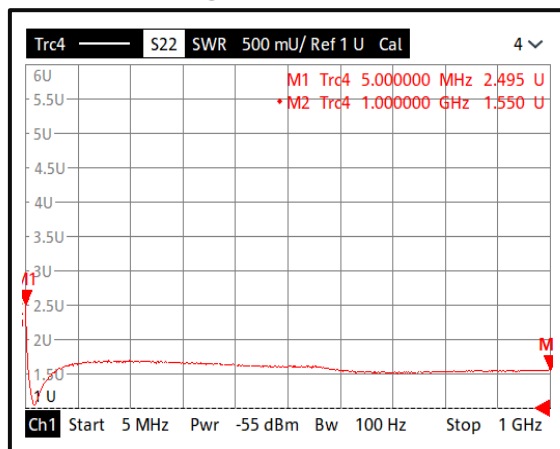
Output VSWR@+25°C (0.005-1GHz)
