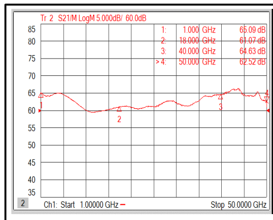
Gain@+25°C (1-50GHz)
