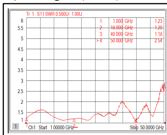
Input VSWR@-40°C (1-50GHz)
