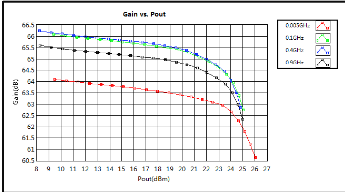
Gain vs. Output Power (0.005-0.9GHz)
