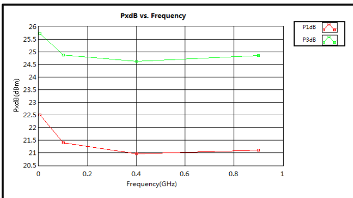
PndB vs. Frequency (0.005-0.9GHz)
