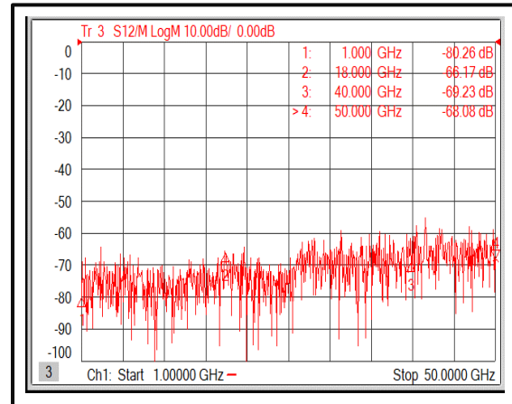
Isolation@-40°C (1-50GHz)
