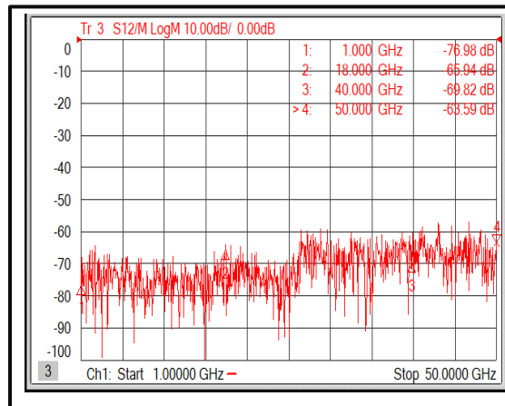
Isolation@+25°C (1-50GHz)
