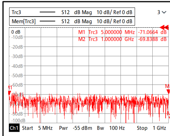
Isolation@-40°C (0.005-1GHz)
