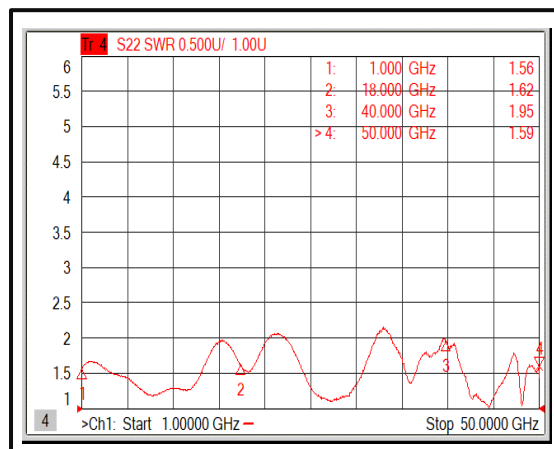
Output VSWR@+25°C (1-50GHz)
