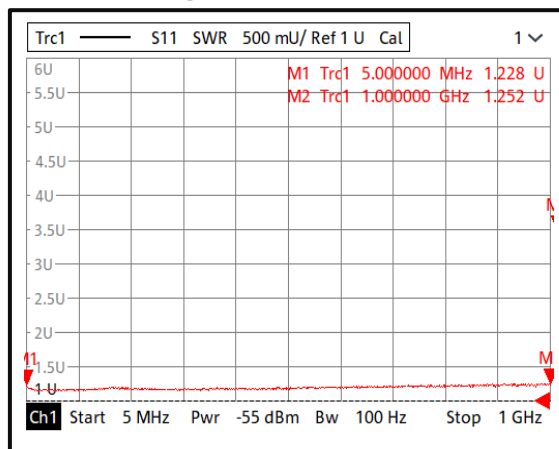
Input VSWR@+85°C (0.005-1GHz)
