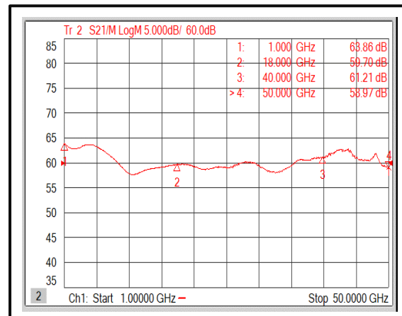
Gain@+85°C (1-50GHz)
