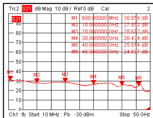
Gain vs. Frequency @-10°C
