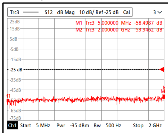
Isolation@-40°C (0.005-2GHz)
