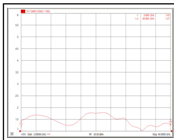
Input VSWR@+25°C (2-40GHz)
