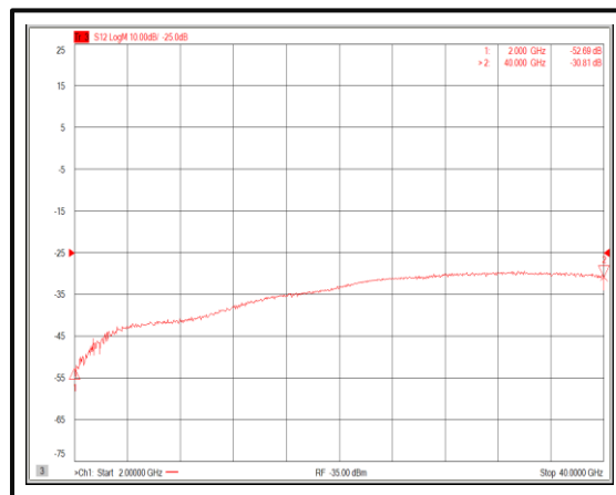
Isolation@+25°C (2-40GHz)
