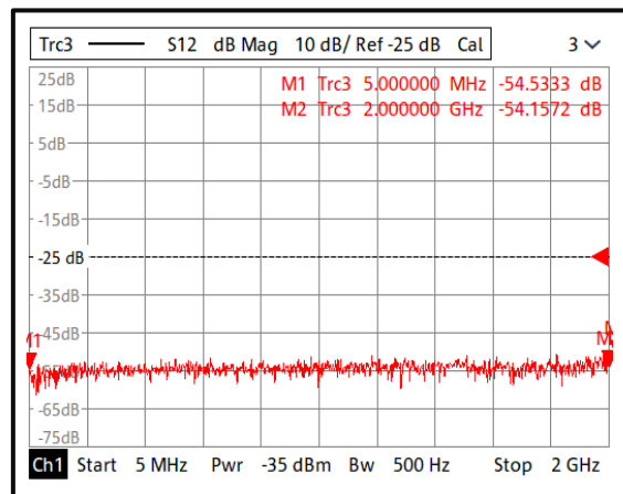
Isolation@+25°C (0.005-2GHz)
