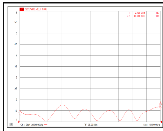
Output VSWR@-40°C (2-40GHz)
