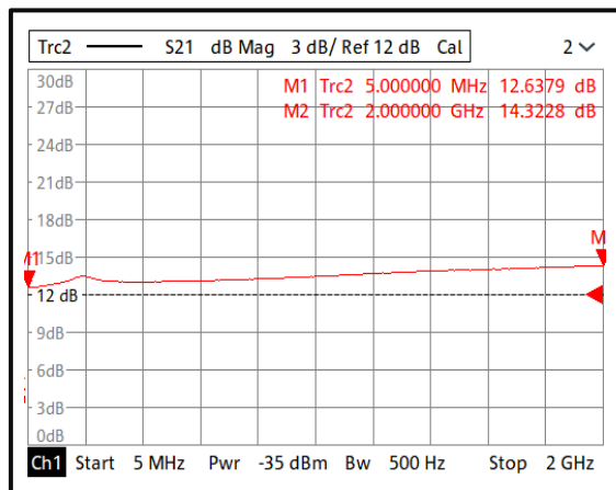
Gain@+25°C (0.005-2GHz)
