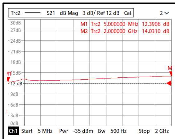
Gain@+85°C (0.005-2GHz)
