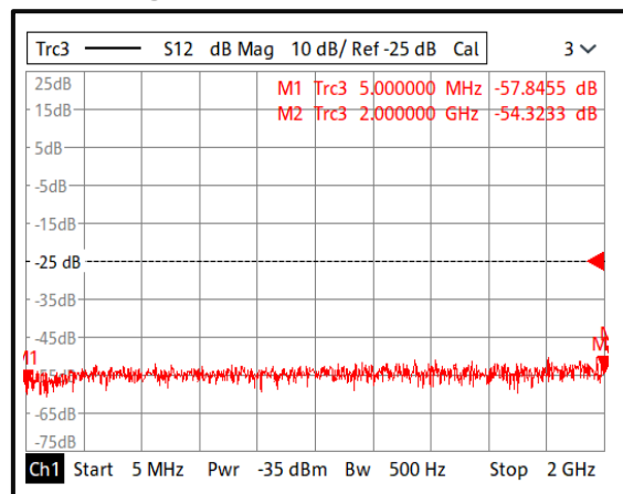
Isolation@+85°C (0.005-2GHz)
