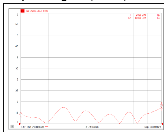
Output VSWR@+85°C (2-40GHz)
