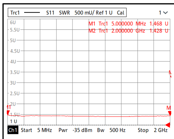
Input VSWR@+25°C (0.005-2GHz)
