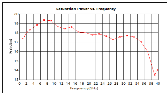
Saturation Power vs. Frequency (1-40GHz)
