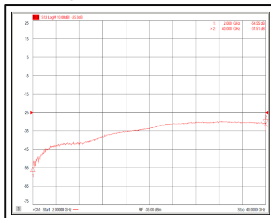
Isolation@+85°C (2-40GHz)
