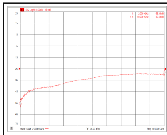
Isolation@-40°C (2-40GHz)
