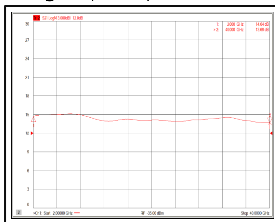
Gain@-40°C (2-40GHz)
