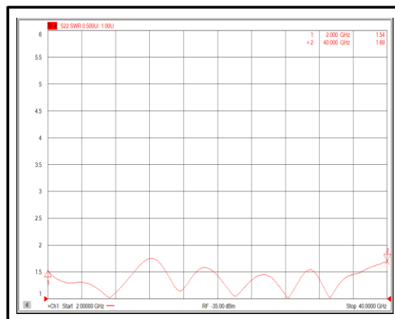
Output VSWR@+25°C (2-40GHz)
