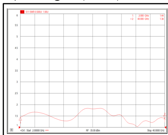
Input VSWR@-40°C (2-40GHz)
