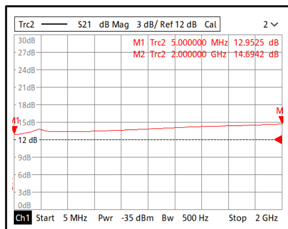
Gain@-40°C (0.005-2GHz)
