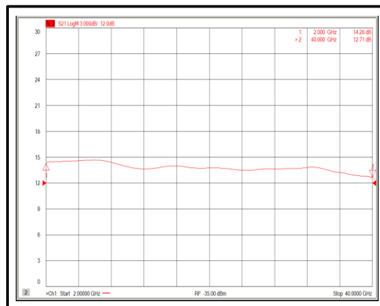
Gain@+25°C (2-40GHz)
