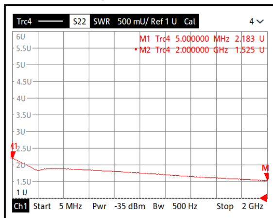
Output VSWR@+25°C (0.005-2GHz)
