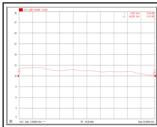
Gain@+85°C (2-40GHz)
