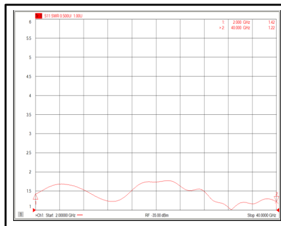
Input VSWR@+85°C (2-40GHz)
