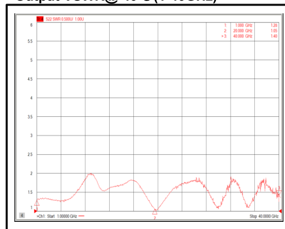
Output VSWR@-40°C (1-40GHz)
