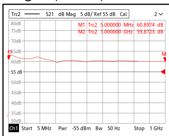
Gain@+85°C (0.005-1GHz)
