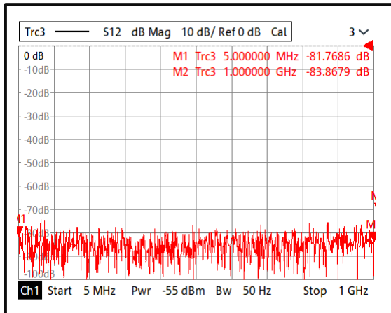
Isolation@+85°C (0.005-1GHz)
