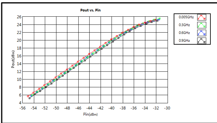
Pout vs. Pin (0.005-0.9GHz)
