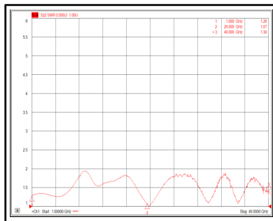
Output VSWR@+25°C (1-40GHz)
