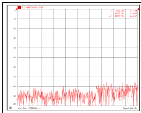
Isolation@+25°C (1-40GHz)
