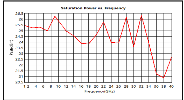
Saturation Power vs. Frequency (1-40GHz)
