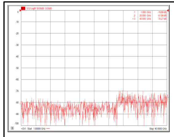
Isolation@+85°C (1-40GHz)
