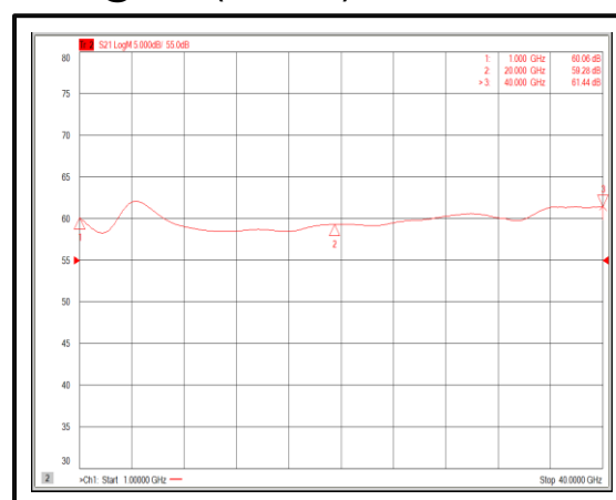
Gain@+85°C (1-40GHz)
