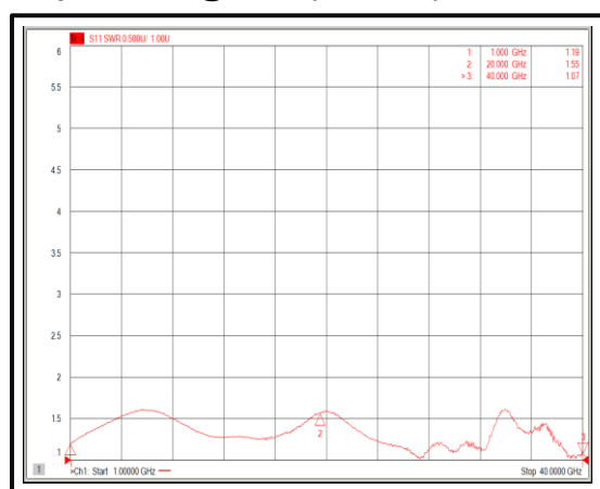
Input VSWR@+25°C (1-40GHz)
