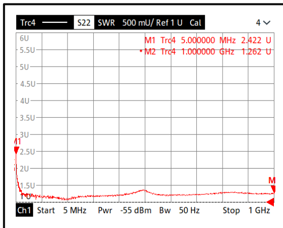
Output VSWR@+85°C (0.005-1GHz)
