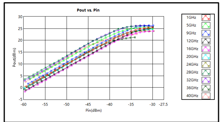
Pout vs. Pin (1-40GHz)
