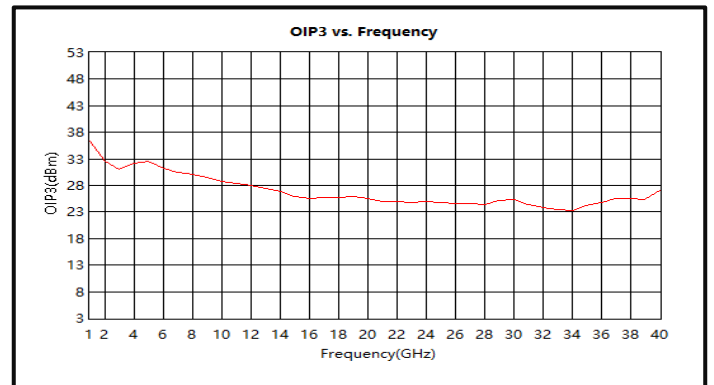
Output Third Order Intercept (OIP3) (1-40GHz)
