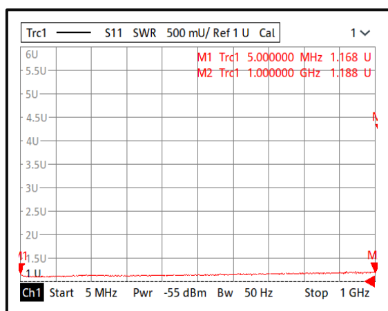
Input VSWR@+25°C (0.005-1GHz)
