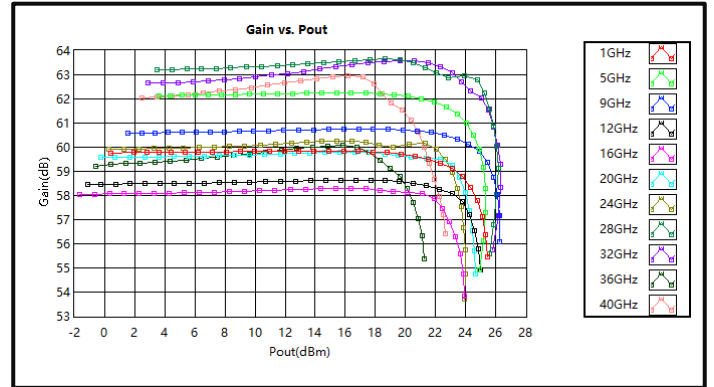
Gain vs. Output Power (1-40GHz)
