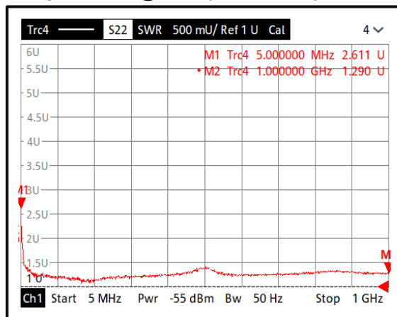
Output VSWR@-40°C (0.005-1GHz)
