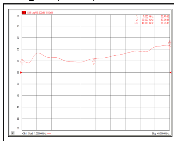
Gain@-40°C (1-40GHz)
