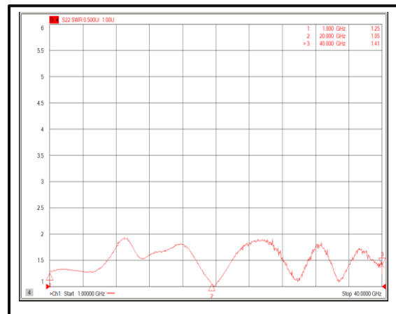
Output VSWR@+85°C (1-40GHz)
