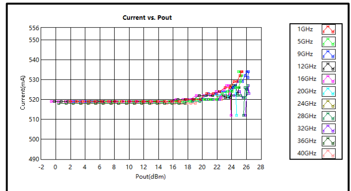
Current vs. Pout (1-40GHz)
