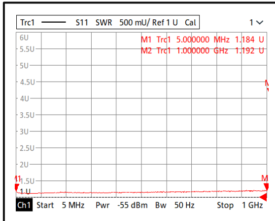
Input VSWR@+85°C (0.005-1GHz)
