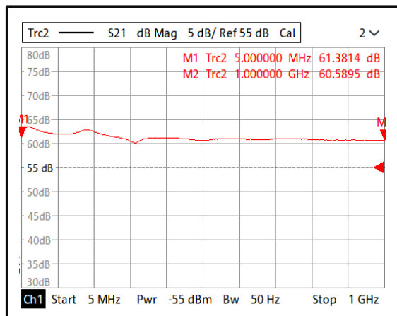
Gain@+25°C (0.005-1GHz)
