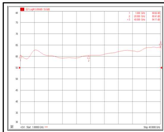
Gain@+25°C (1-40GHz)
