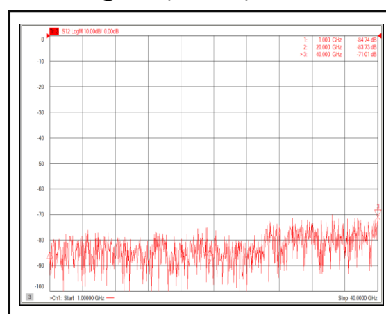
Isolation@-40°C (1-40GHz)
