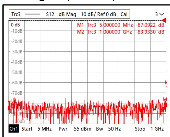
Isolation@-40°C (0.005-1GHz)
