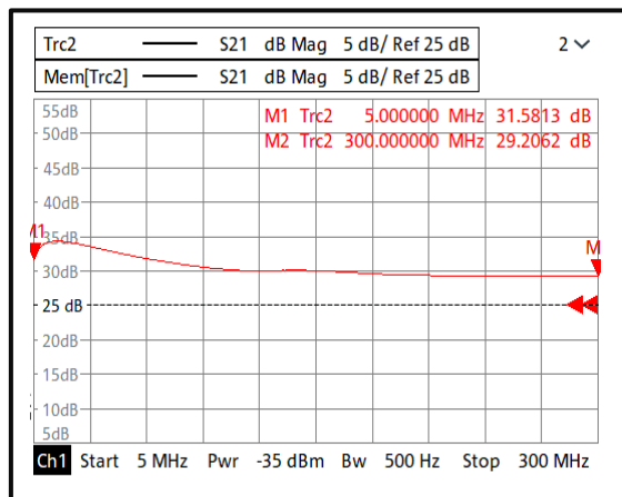
Gain@+25°C (0.005-0.3GHz)
