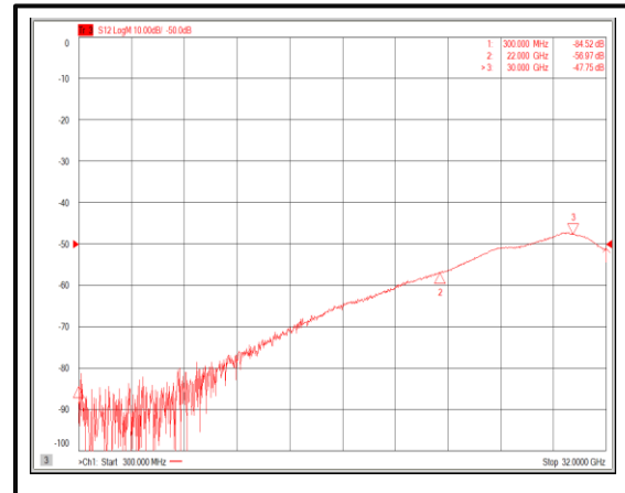
Isolation@-40°C (0.3-30GHz)
