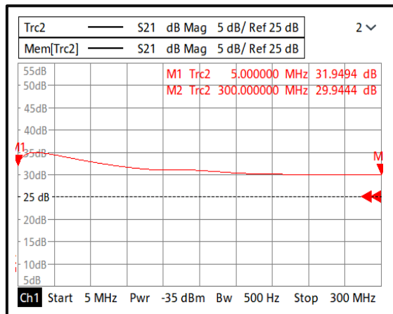
Gain@-40°C (0.005-0.3GHz)
