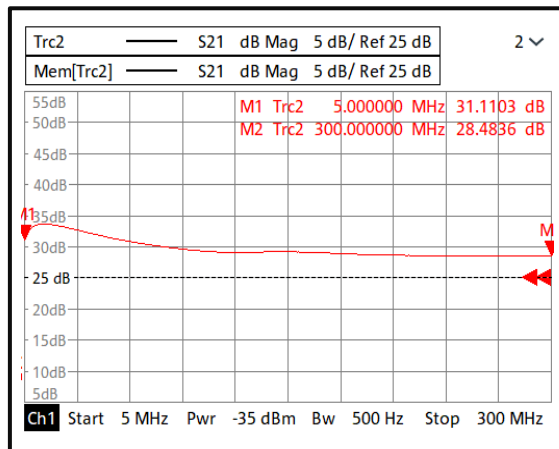
Gain@+85°C (0.005-0.3GHz)
