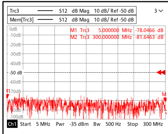
Isolation@-40°C (0.005-0.3GHz)
