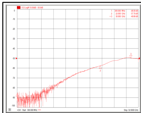
Isolation@+85°C (0.3-30GHz)
