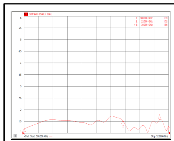
Input VSWR@+25°C (0.3-30GHz)
