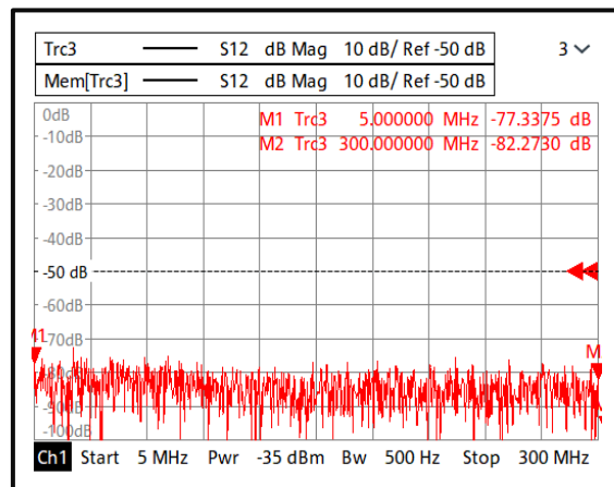
Isolation@+85°C (0.005-0.3GHz)
