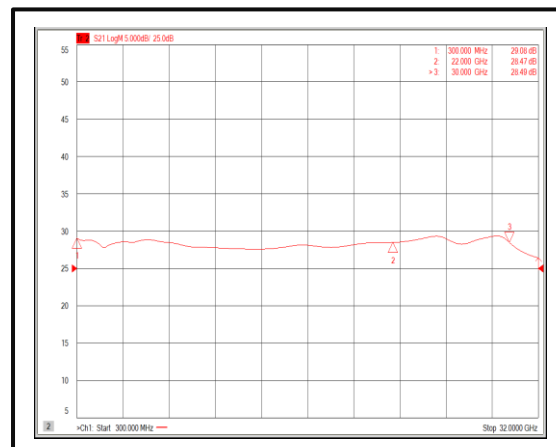
Gain@+25°C (0.3-30GHz)
