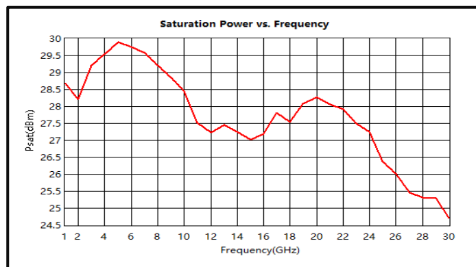
Saturation Power vs. Frequency (1-30GHz)
