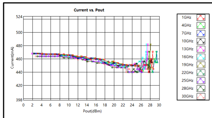
Current vs. Pout (1-30GHz)
