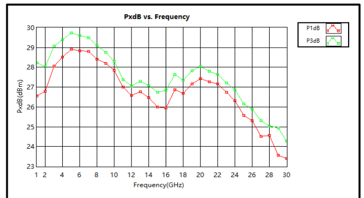
PndB vs. Frequency (1-30GHz)
