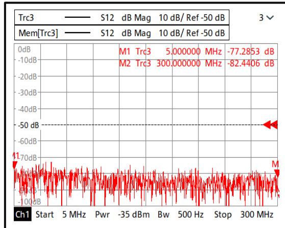
Isolation@+25°C (0.005-0.3GHz)
