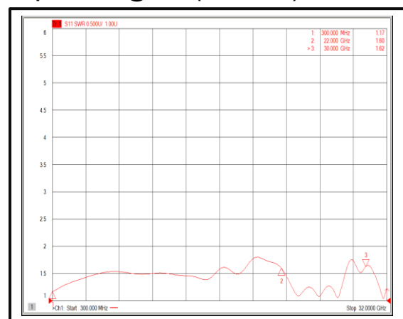
Input VSWR@-40°C (0.3-30GHz)
