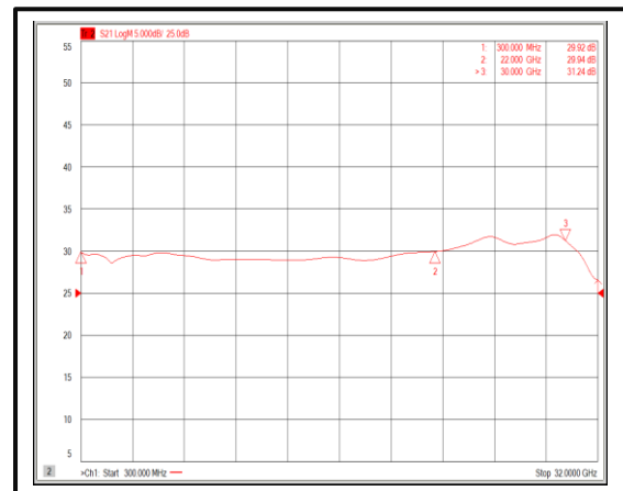
Gain@-40°C (0.3-30GHz)
