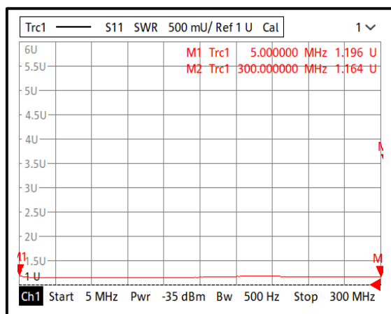
Input VSWR@-40°C (0.005-0.3GHz)
