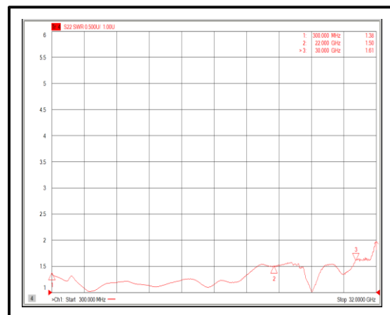
Output VSWR@+25°C (0.3-30GHz)
