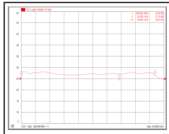
Gain@+85°C (0.3-30GHz)
