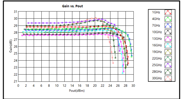
Gain vs. Output Power (1-30GHz)
