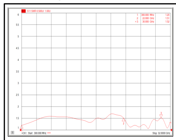
Input VSWR@+85°C (0.3-30GHz)
