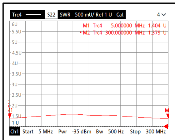
Output VSWR@+25°C (0.005-0.3GHz)
