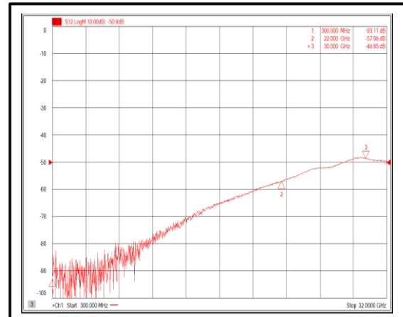
Isolation@+25°C (0.3-30GHz)
