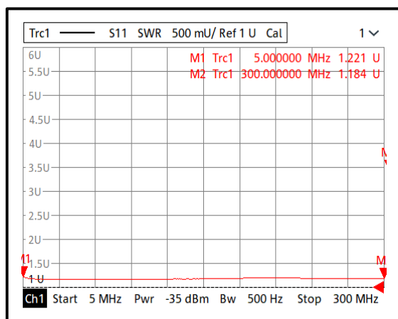
Input VSWR@+25°C (0.005-0.3GHz)
