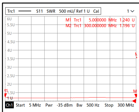
Input VSWR@+85°C (0.005-0.3GHz)
