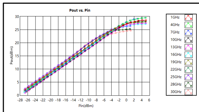
Pout vs. Pin (1-30GHz)
