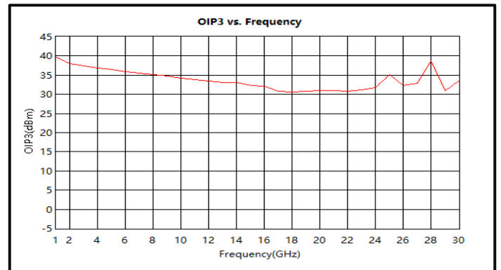
Output Third Order Intercept (OIP3) (1-30GHz)
