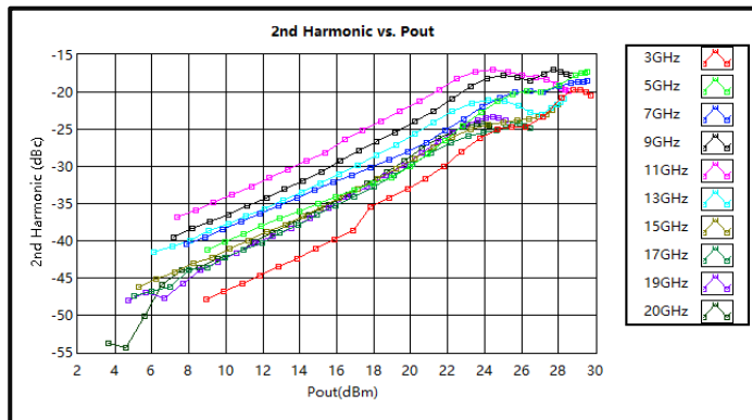
2nd Harmonic Wave Output Power (3-20GHz)
