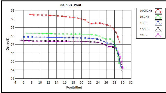
Gain vs. Output Power (0.005-2GHz)
