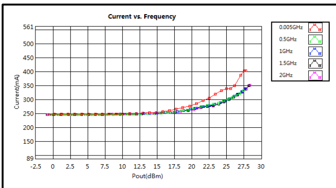
Current vs. Frequency (0.005-2GHz)
