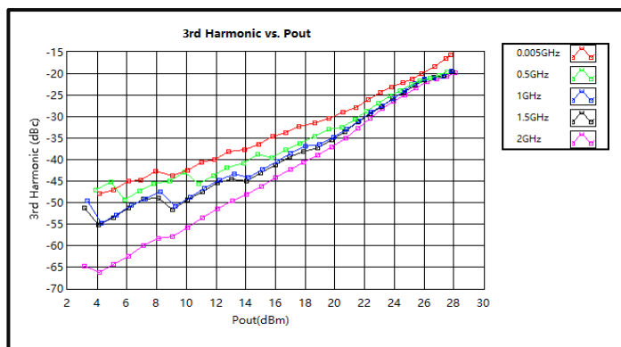
3rd Harmonic Wave Output Power (0.005-2GHz)
