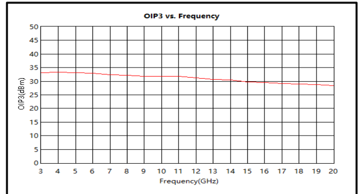
Output Third Order Intercept (OIP3) (3-20GHz)
