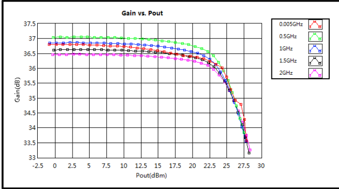
Gain vs. Output Power (0.005-2GHz)
