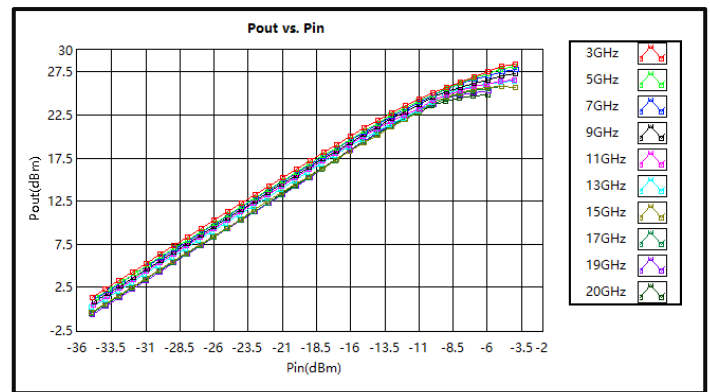
Pout vs. Pin (3-20GHz)
