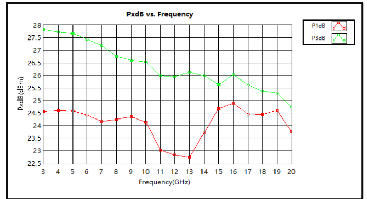
P1dB & P3dB vs. Frequency (3-20GHz)
