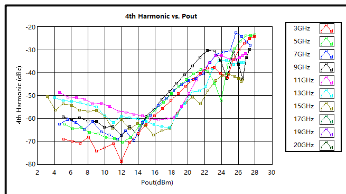
4th Harmonic Wave Output Power (3-20GHz)
