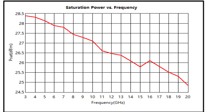
Saturation Power vs. Frequency (3-20GHz)
