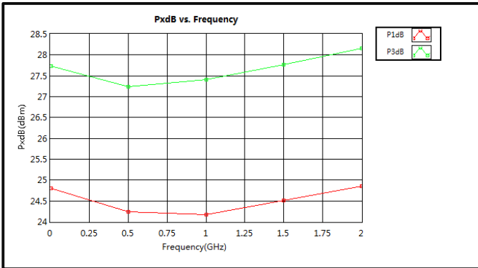
P1dB & P3dB vs. Frequency (0.005-2GHz)
