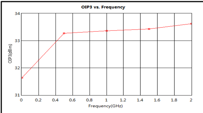
Output Third Order Intercept (OIP3) (0.005-2GHz)
