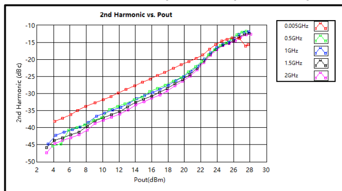
2nd Harmonic Wave Output Power (0.005-2GHz)
