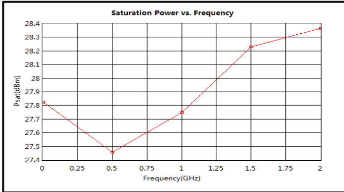
Saturation Power vs. Frequency (0.005-2GHz)
