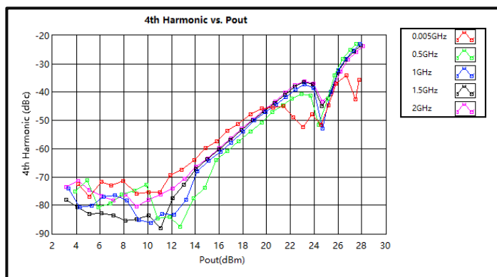
4th Harmonic Wave Output Power (0.005-2GHz)
