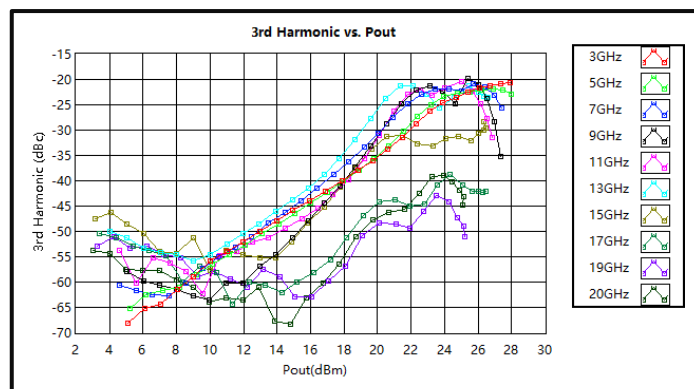
3rd Harmonic Wave Output Power (3-20GHz)
