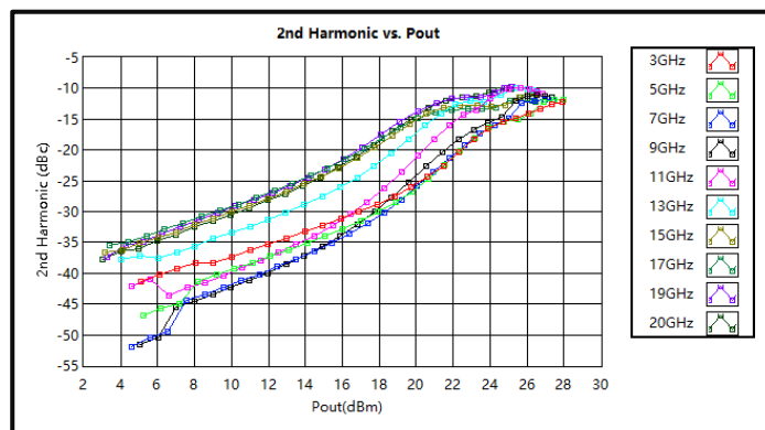
2nd Harmonic Wave Output Power (3-20GHz)
