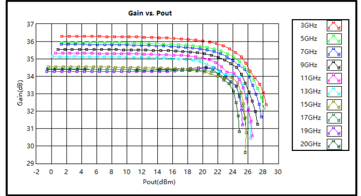
Gain vs. Output Power (3-20GHz)
