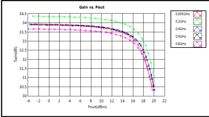
Gain vs. Output Power (0.005-0.8GHz)
