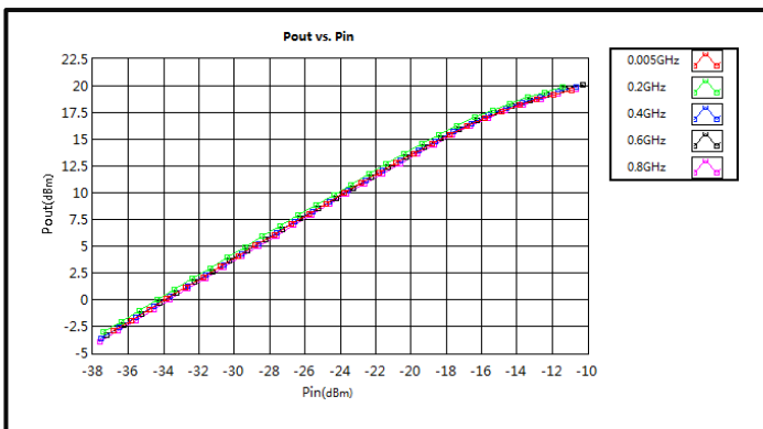
Pout vs. Pin (0.005-0.8GHz)
