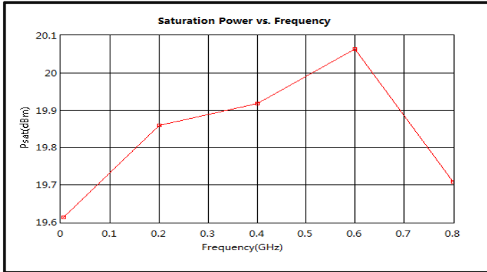
Saturation Power vs. Frequency (0.005-0.8GHz)
