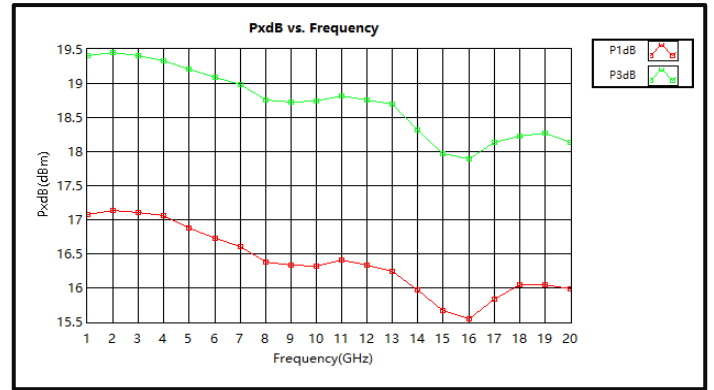
P1dB & P3dB vs. Frequency (1-20GHz)
