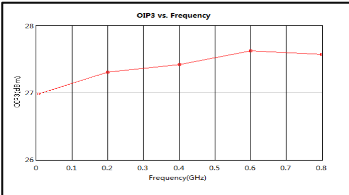
Output Third Order Intercept (OIP3) (0.005-0.8GHz)
