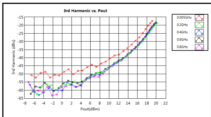
3rd Harmonic Wave Output Power (0.005-0.8GHz)
