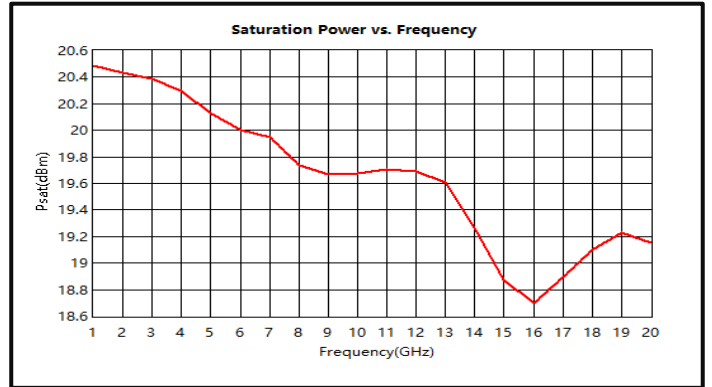
Saturation Power vs. Frequency (1-20GHz)
