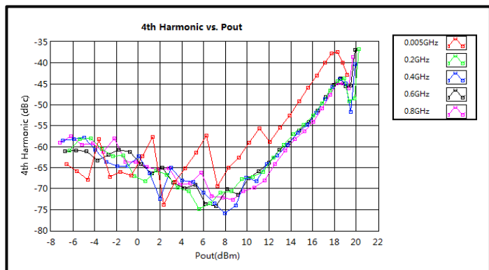
4th Harmonic Wave Output Power (0.005-0.8GHz)
