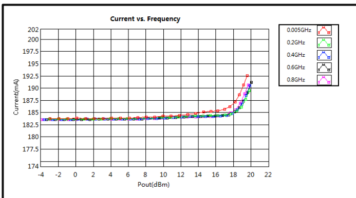
Current vs. Frequency (0.005-0.8GHz)
