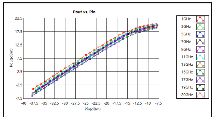
Pout vs. Pin (1-20GHz)
