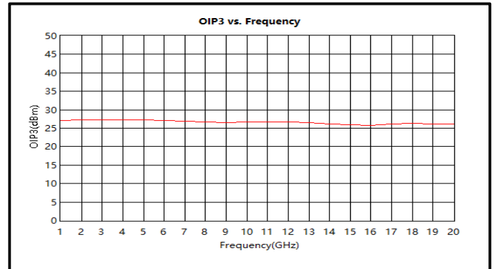
Output Third Order Intercept (OIP3) (1-20GHz)
