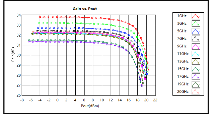
Gain vs. Output Power (1-20GHz)
