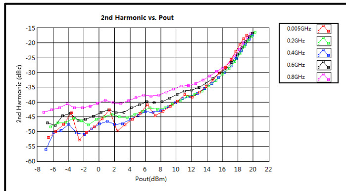
2nd Harmonic Wave Output Power (0.005-0.8GHz)
