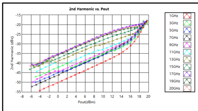
2nd Harmonic Wave Output Power (1-20GHz)
