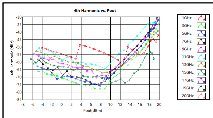
4th Harmonic Wave Output Power (1-20GHz)
