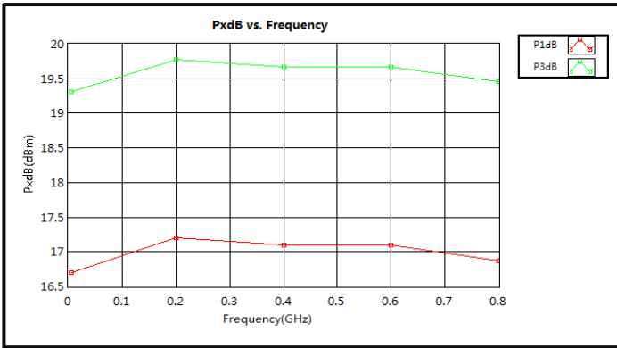
P1dB & P3dB vs. Frequency (0.005-0.8GHz)
