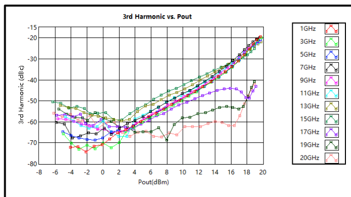
3rd Harmonic Wave Output Power (1-20GHz)
