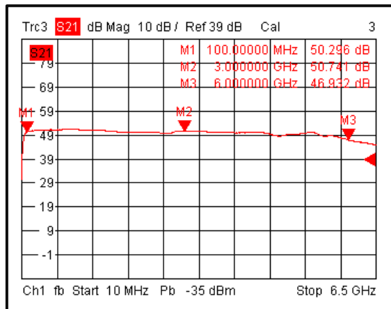
Gain@+85°C
