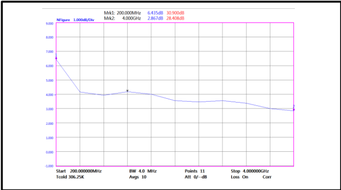
Noise Figure(0.2-4GHz)
