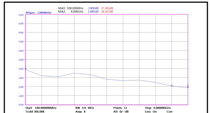
Noise Figure (100MHz-4GHz)
