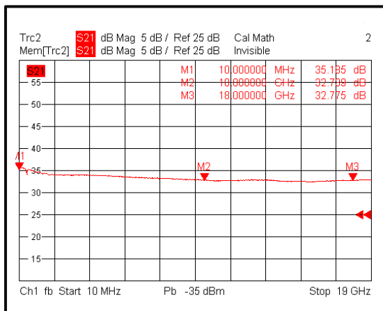
Gain@+85°C
