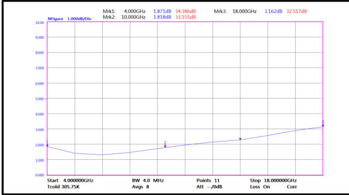
Noise Figure (4GHz-18GHz)
