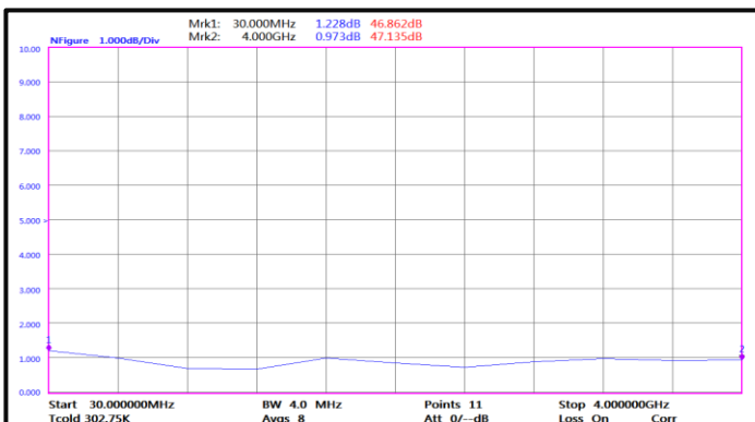
Noise Figure(0.03GHz-4GHz)
