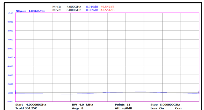
Noise Figure(4GHz-6GHz)
