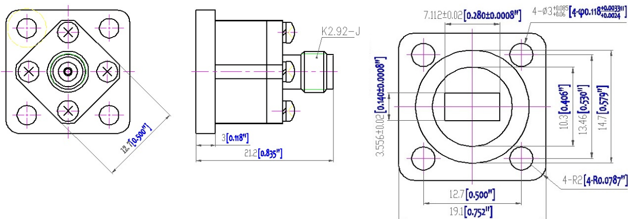
2.92mm Male Connector
