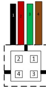
Switch Control Cable
