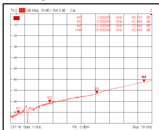
Isolation @+85°C
