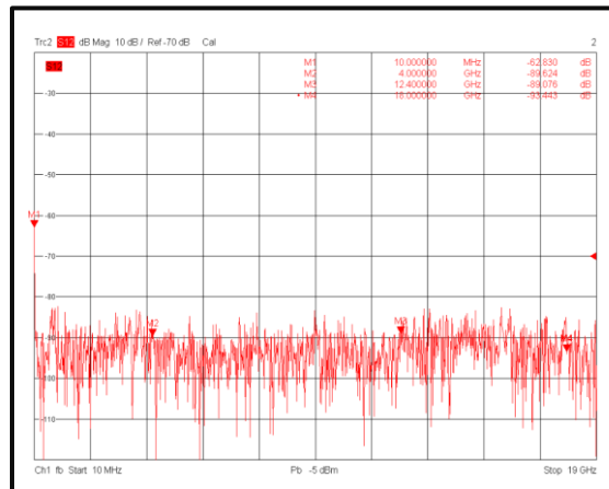
Isolation @-20°C
