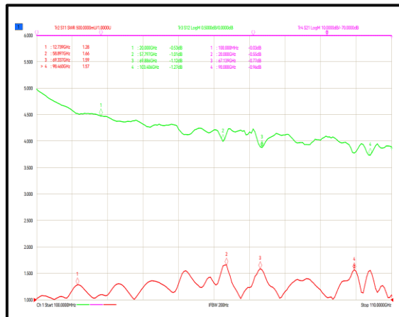
Insertion Loss & VSWR
