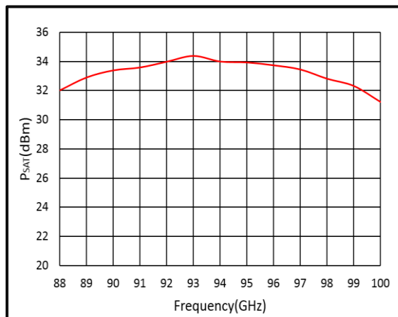
Saturation Power vs. Frequency CW
