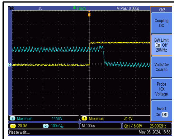
The AMP-Enable Rise Time is 100 us @+25°C
