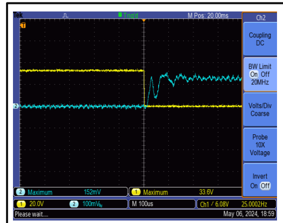
The AMP-Disable Fall Time is 100 us @+25°C
