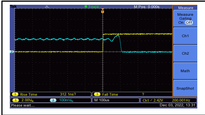
The Drain-Disable Rise Time is 100 \mu s
