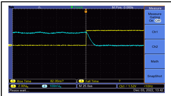
The Gate-Disable Rise Time is 20 \mu s
