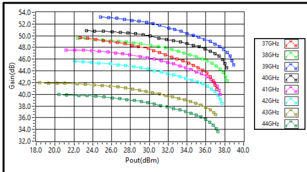
Gain vs. Output power @+25 °C (CW Signal)
