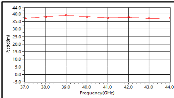
Psat vs. Frequency @+25°C (CW Signal)
