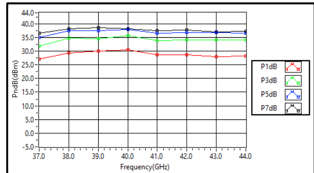
PndB vs. Frequency +25°C (CW Signal)
