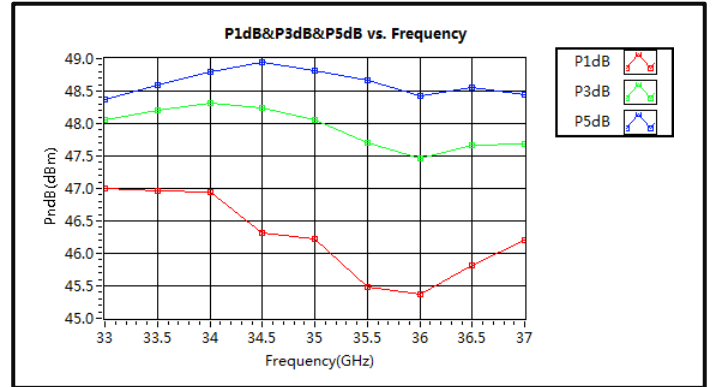
PndB vs Frequency *Pulse
