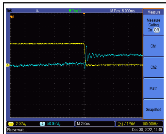
The Switching Fall Time is 250 ns @+25°C
