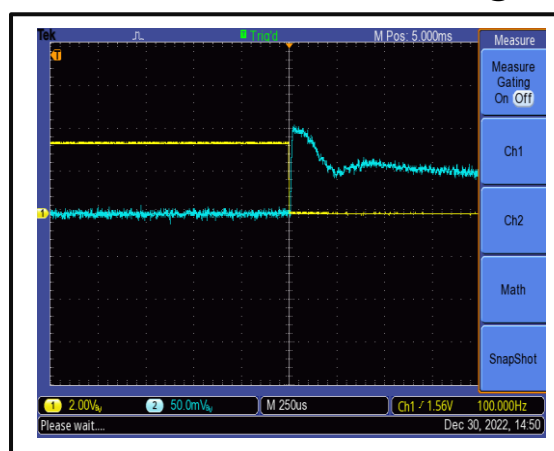
The Drain-Disable Fall Time is 500 us @+25°C
