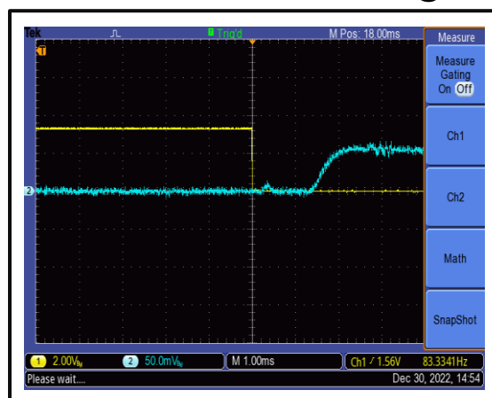
The Gate-Enable Fall Time is 2000us@+25°C
