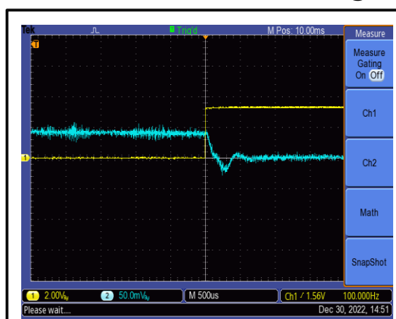
The Drain-Enable Rise Time is 500 us @+25°C
