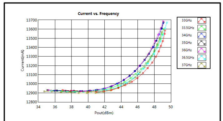
Current vs. Pout *Pulse
