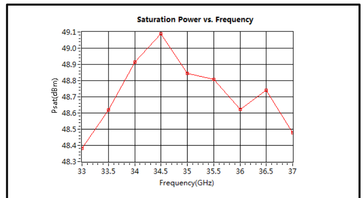
Saturation Power vs. Frequency *Pulse
