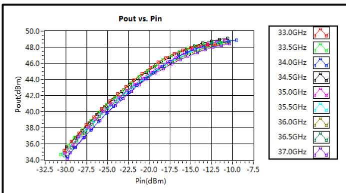
Pout vs. Pin *Pulse
