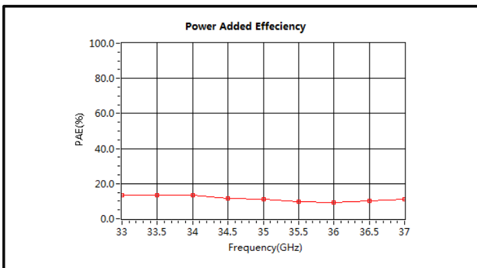
Power Added Efficiency *Pulse
