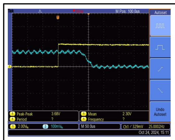
The Drains-Disable Fall Time is 100 us @+25°C
