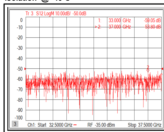
Isolation @ -40°C
