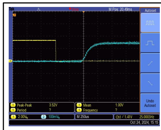
The Gates-Rise Time is 750 us @+25°C
