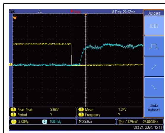
The Drains-Enable Rise Time is 25 us @+25°C
