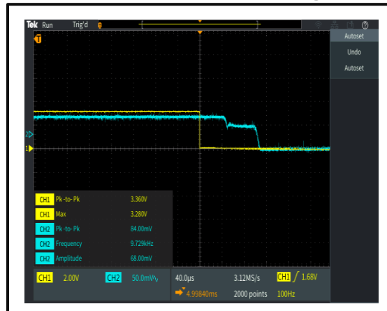
The Switching Fall Time is 100 us @+25°C
