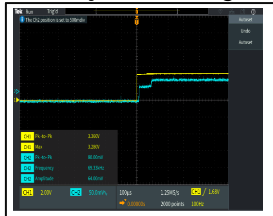
The Switching Rise Time is 100 us @+25°C
