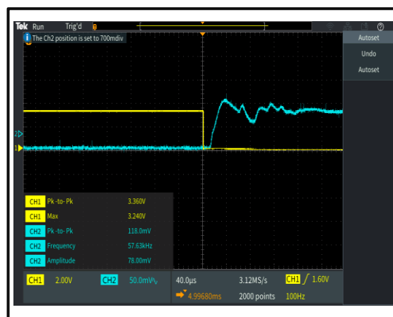
The Drain-Disable Fall Time is 40 us @+25°C
