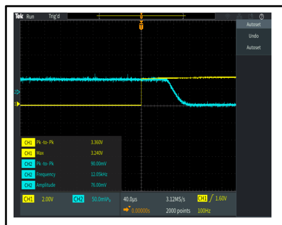
The Drain-Enable Rise Time is 100 us @+25°C
