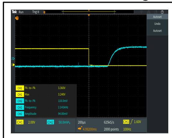
The Gate-Enable Fall Time is 600 us @+25°C
