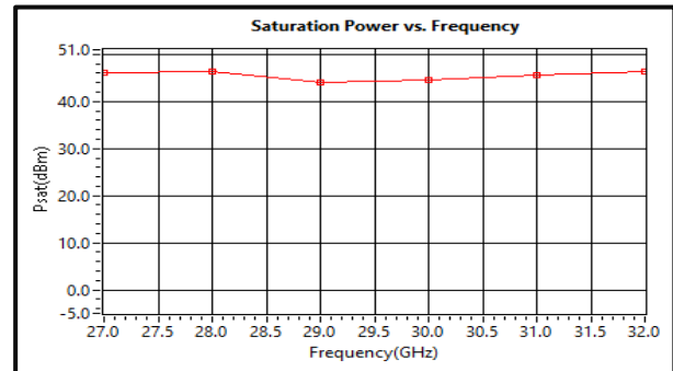
Saturation Power vs. Frequency
