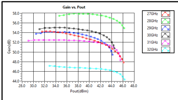
Gain vs. Pout
