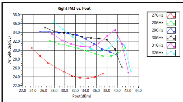
Right IM3 vs. Pout
