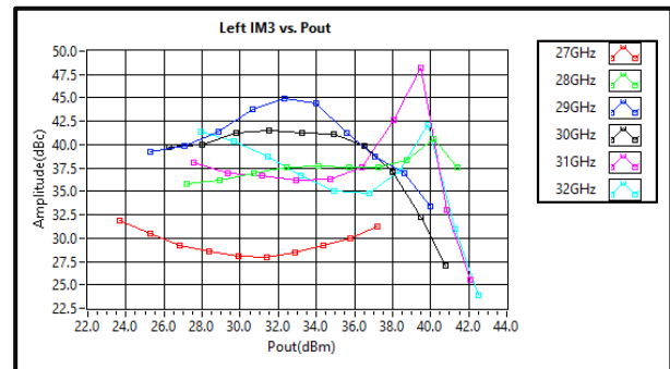
Left IM3 vs. Pout
