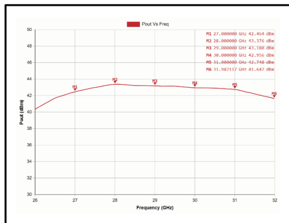
Pout vs Frequency @ +25°C
