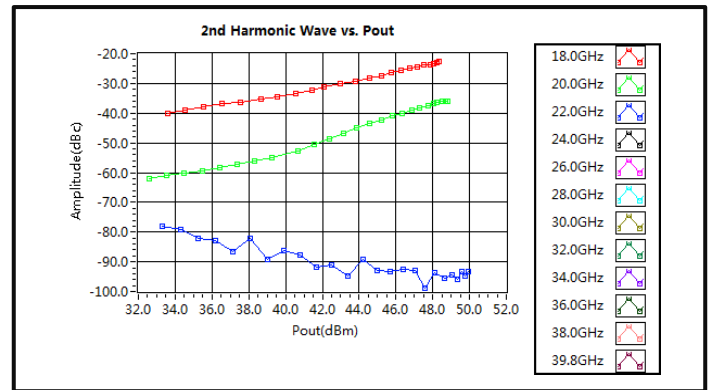
2nd Harmonic Wave vs. Pout
