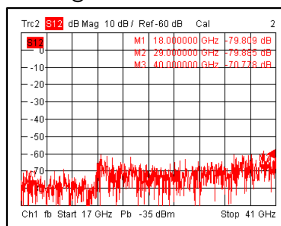
Isolation @ +60°C
