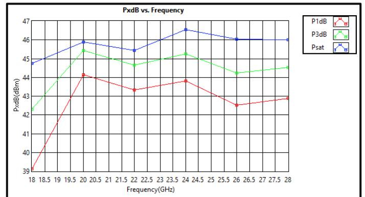
PxdB vs Frequency *Pulse (18-28GHz)
