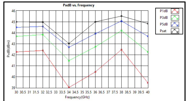
PxdB vs Frequency *Pulse (30-40GHz)
