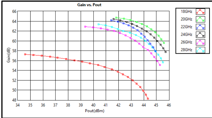
Gain vs Output Power CW (18-28GHz)
