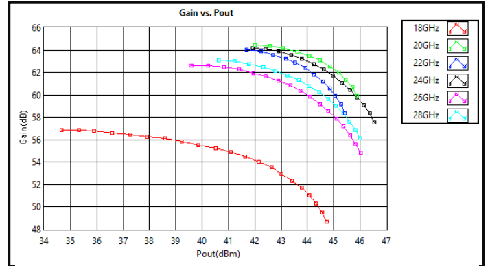
Gain vs Output Power *Pulse (18-28GHz)
