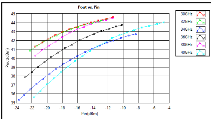
Output vs Input Power CW (30-40GHz)
