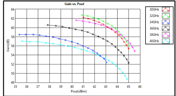
Gain vs Output Power *Pulse (30-40GHz)
