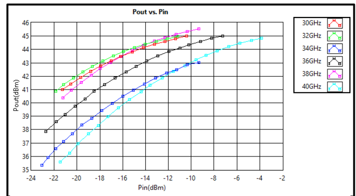
Output vs Input Power *Pulse (30-40GHz)
