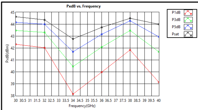
PxdB vs Frequency CW (30-40GHz)
