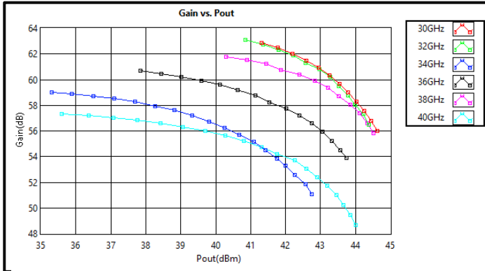
Gain vs Output Power CW (30-40GHz)
