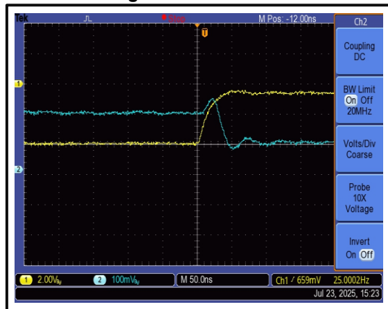
The Switching Rise Time is 100 ns
