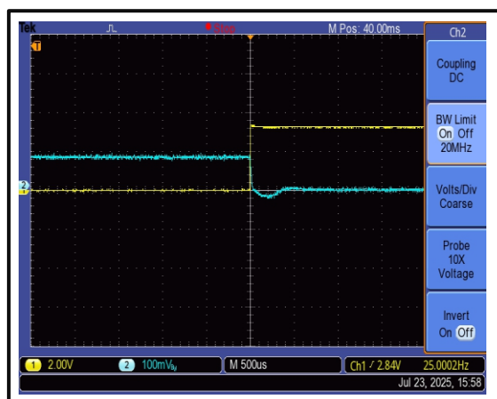
The Gate-Enable Rise Time is 400 us
