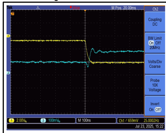
The Switching Fall Time is 100 ns
