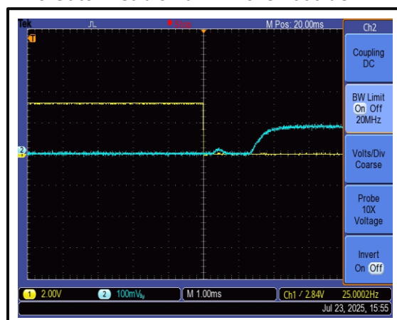
The Gate-Disable Fall Time is 2000 us
