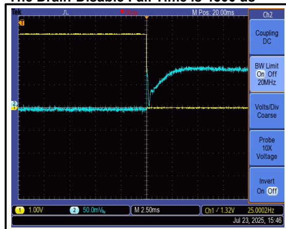
The Drain-Disable Fall Time is 4500 us
