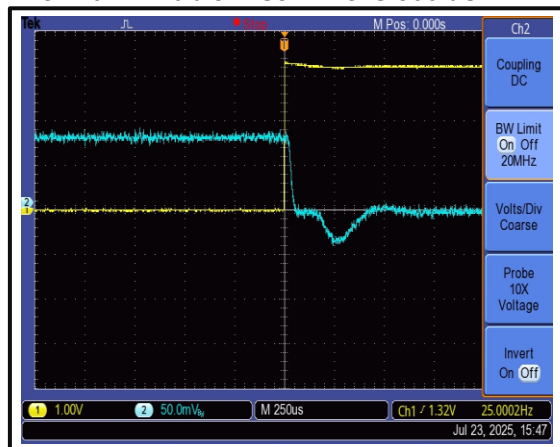
The Drain-Enable Rise Time is 500 us
