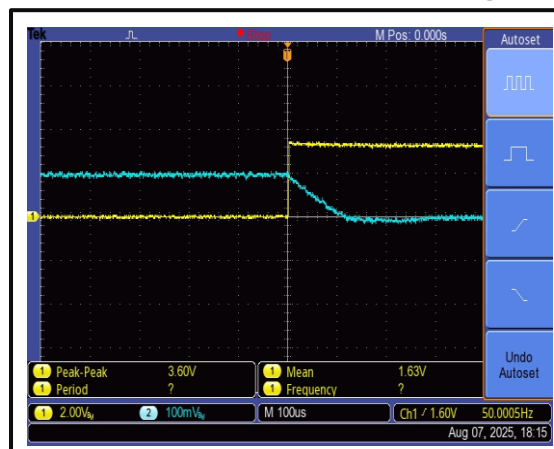
The Gate-Disable Fall Time is 120 us @+25°C
