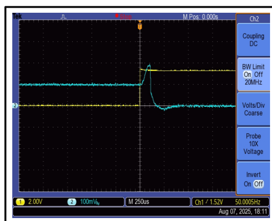
The Drain-Disable Fall Time is 250 us @+25°C
