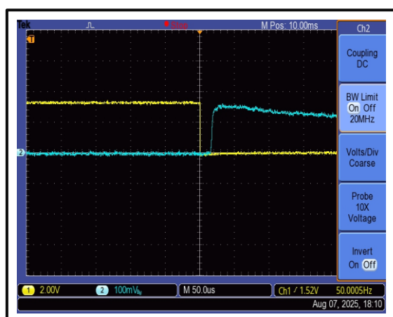
The Drain-Enable Rise Time is 50 us @+25°C
