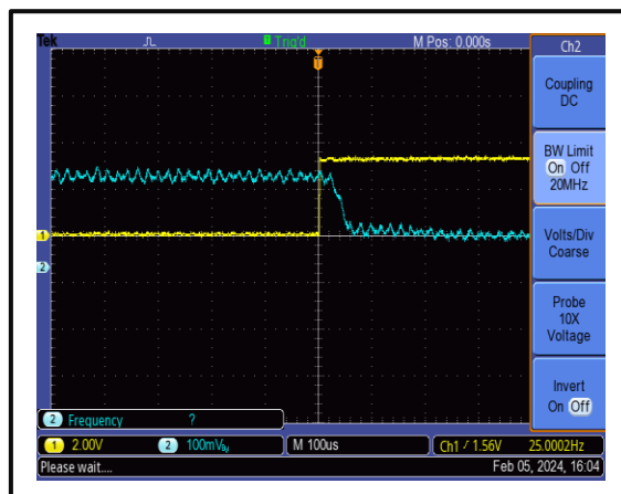
The Gate-Enable Rise Time is 60 us @+25°C
