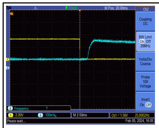
The Gate-Enable Fall Time is 2500 us @+25°C
