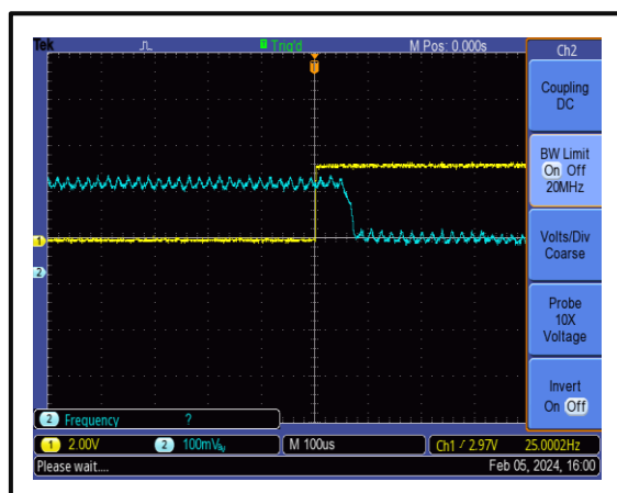
The Drain-Enable Rise Time is 80 us @+25°C
