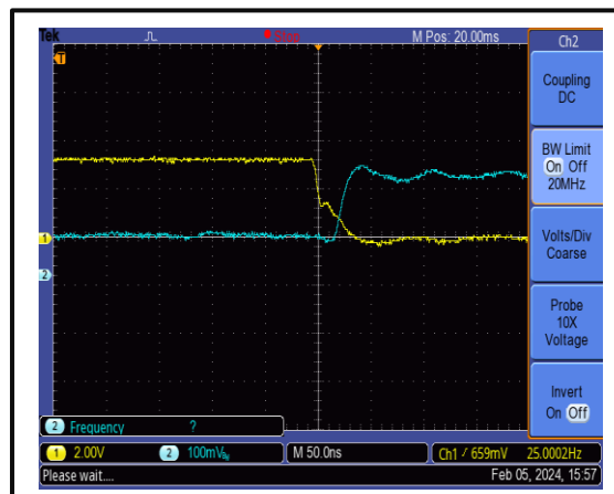
The Switching Fall Time is 50 ns @+25°C
