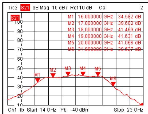
Gain vs. Frequency @-40°C
