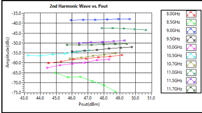
Second Harmonic vs Output Power
