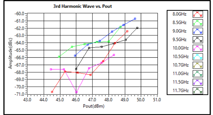
Third Harmonic vs Output Power
