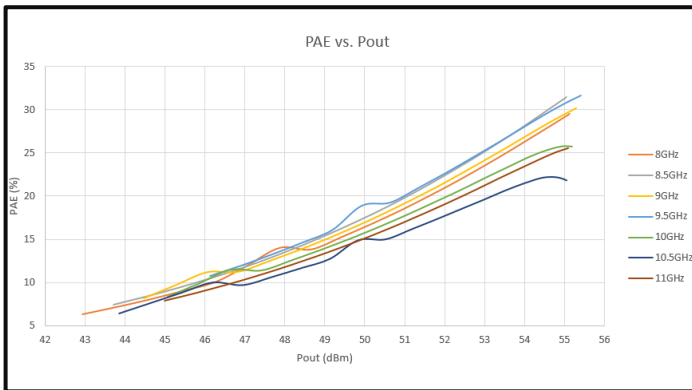
PAE vs Output Power CW
