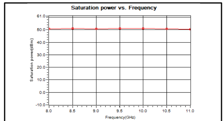
PSat vs Frequency *Pulse
