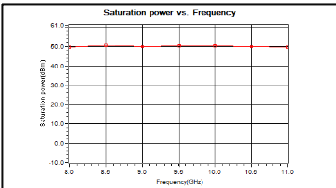
PSat vs Frequency CW
