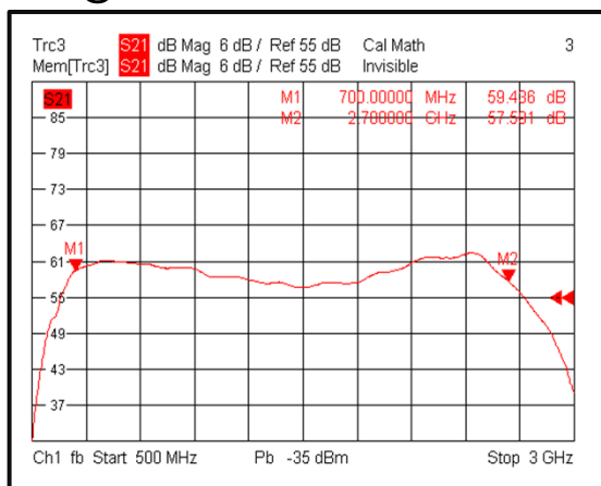
Gain@-40°C
