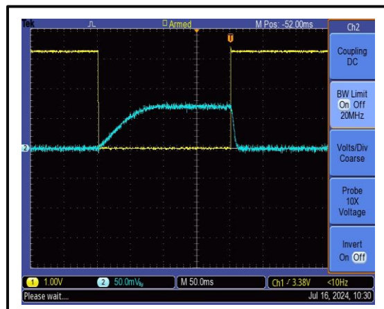
The Drain-Disable Fall Time is 100 ms
