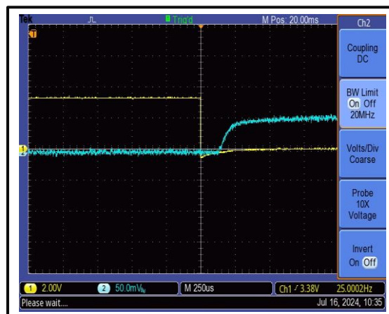
The Gate-Disable Fall Time is 250 us
