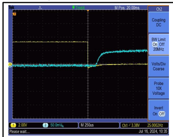
The Gate Open Time is 250 us
