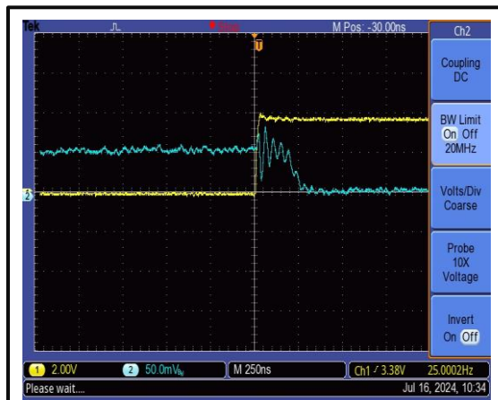
The Gate Closure Time is 250 ns
