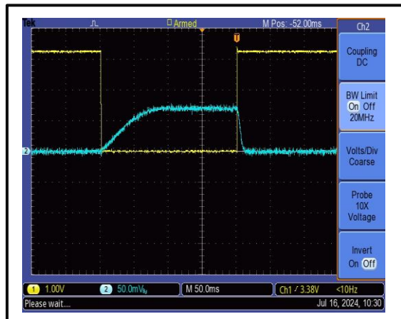
The Drain Open Time is 100 ms
