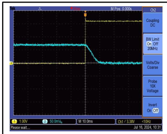
The Drain Closure Time is 10 ms
