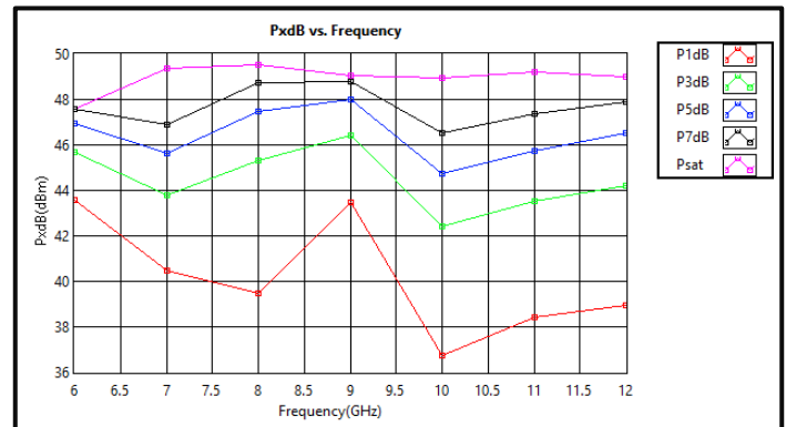
PxdB vs Frequency *Pulse @ +25°C
