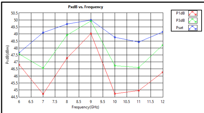
PxdB vs Frequency *Pulse @ -40°C
