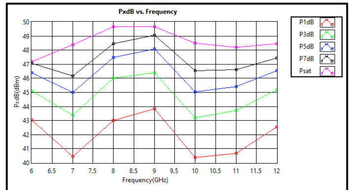
PxdB vs Frequency *Pulse @ +85°C
