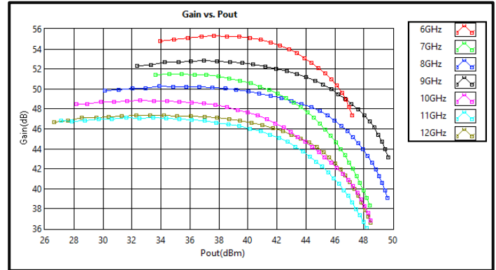
Gain vs Output Power *Pulse @ +85°C
