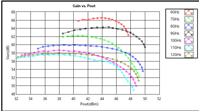
Gain vs Output Power *Pulse @ -40°C
