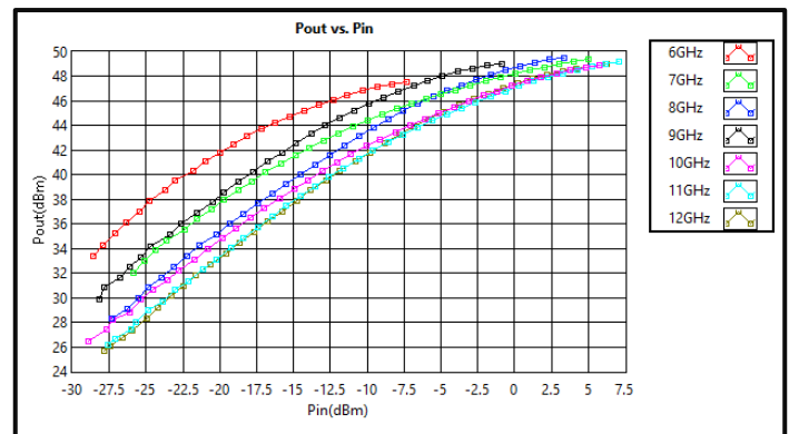
Output vs Input Power *Pulse @ +25°C
