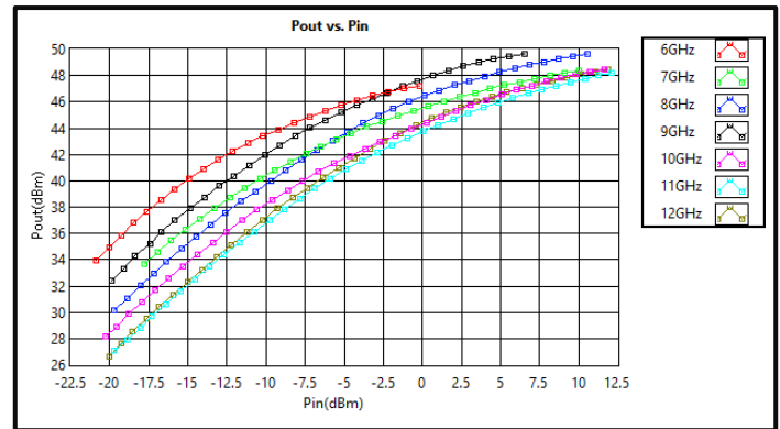
Output vs Input Power *Pulse @ +85°C
