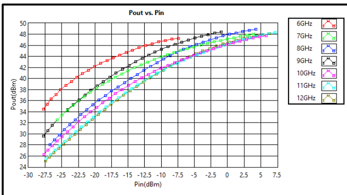
Output vs Input Power CW @ +25°C
