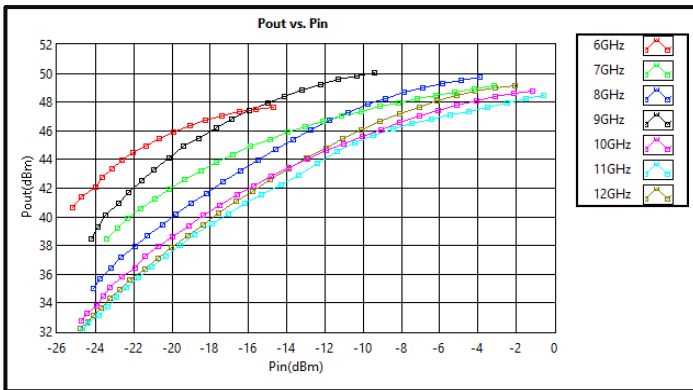
Output vs Input Power *Pulse @ -40°C
