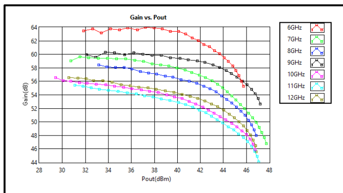
Gain vs Output Power *Pulse @ +25°C
