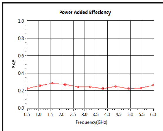
Power Added Efficiency (CW Power)
