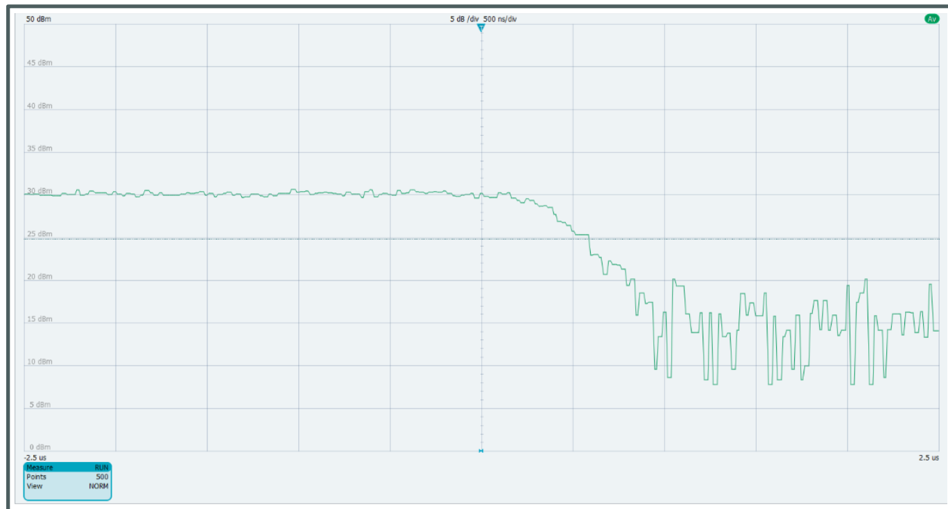
Blanking RF off timing: 30dBm Output Power (500 ns/div)
