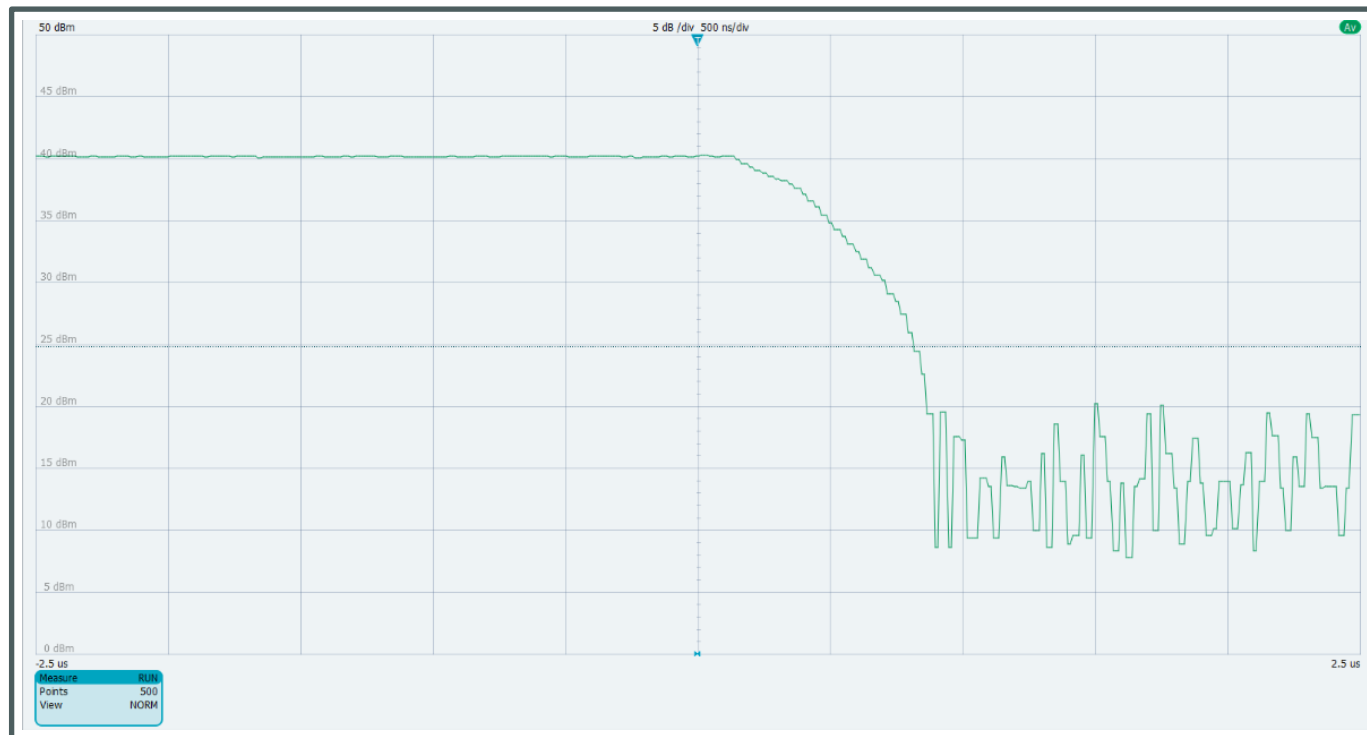
Blanking RF off timing: 40dBm Output Power (500 ns/div)
