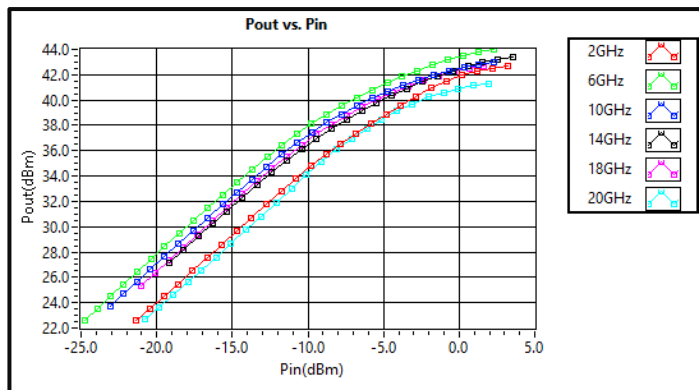
Output vs Input Power CW @ +25°C
