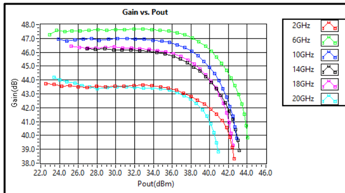
Gain vs Output Power *Pulse @ +25°C
