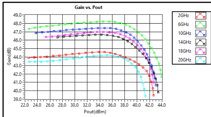
Gain vs Output Power CW @ +25°C
