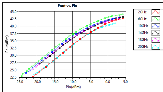
Output vs Input Power *Pulse @ +25°C
