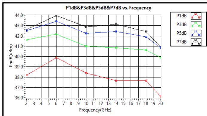
PxdB vs Frequency *Pulse @ +25°C
