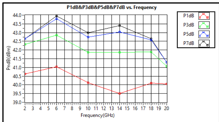
PxdB vs Frequency CW @ +25°C
