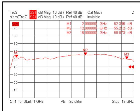
Gain @ +70°C
