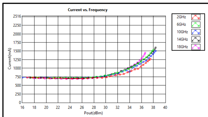
Current vs Output Power (+24DC)
