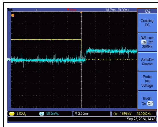
The Gates Fall Time is 1 ms @+25°C
