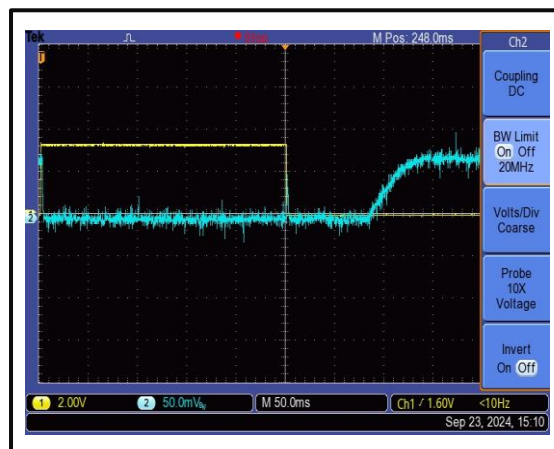
The Drains Fall Time is 150 ms @+25°C
