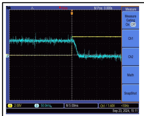
The Drains Rise Time is 2 ms @+25°C
