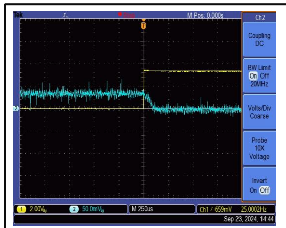
The Gates Rise Time is 100 us @+25°C
