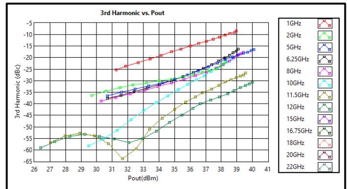
3 rd Harmonic
