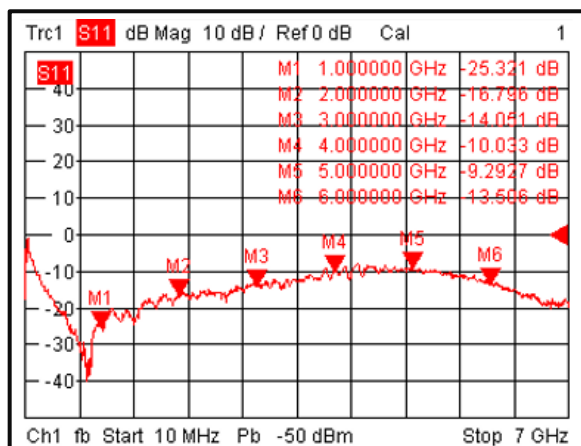
Input Return Loss @+80°C
