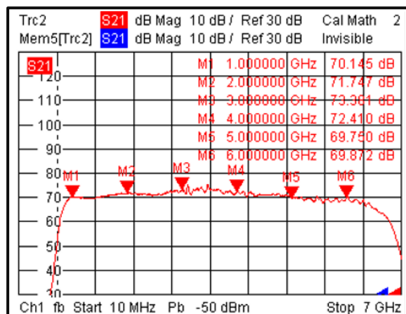
Gain vs. Frequency @-40°C With 15dB Attenuation
