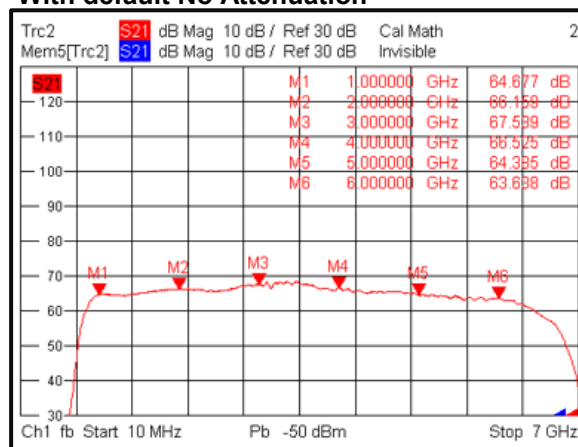
Gain vs. Frequency @+25°C With default No Attenuation
