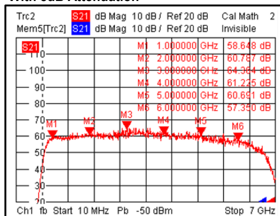
Gain vs. Frequency @+80°C With 5dB Attenuation
