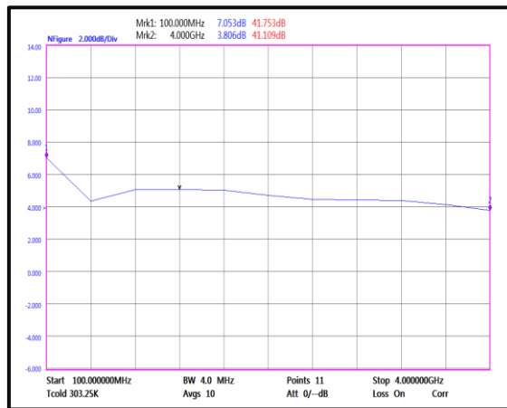
Noise Figure(0.1-4GHz)
