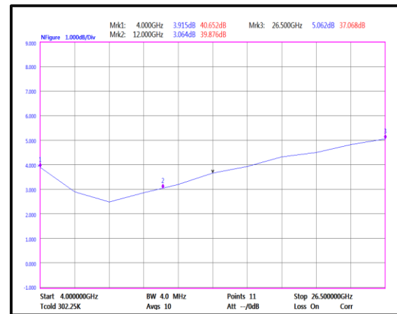
Noise Figure(4-26.5GHz)
